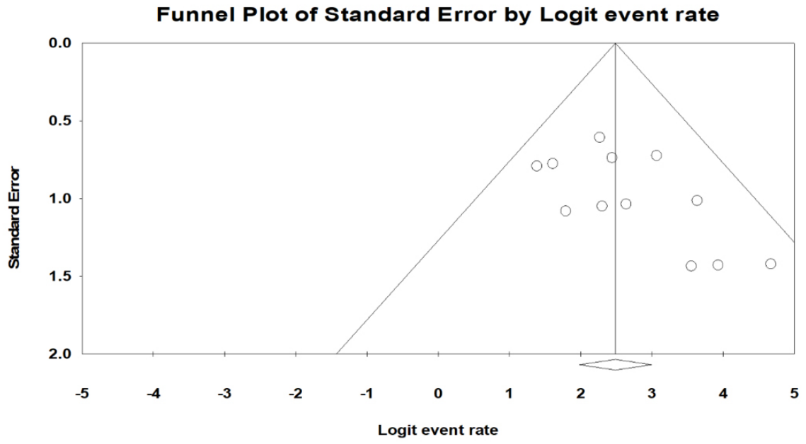
Supplementary Fig. 8. Funnel plot for publication bias.
