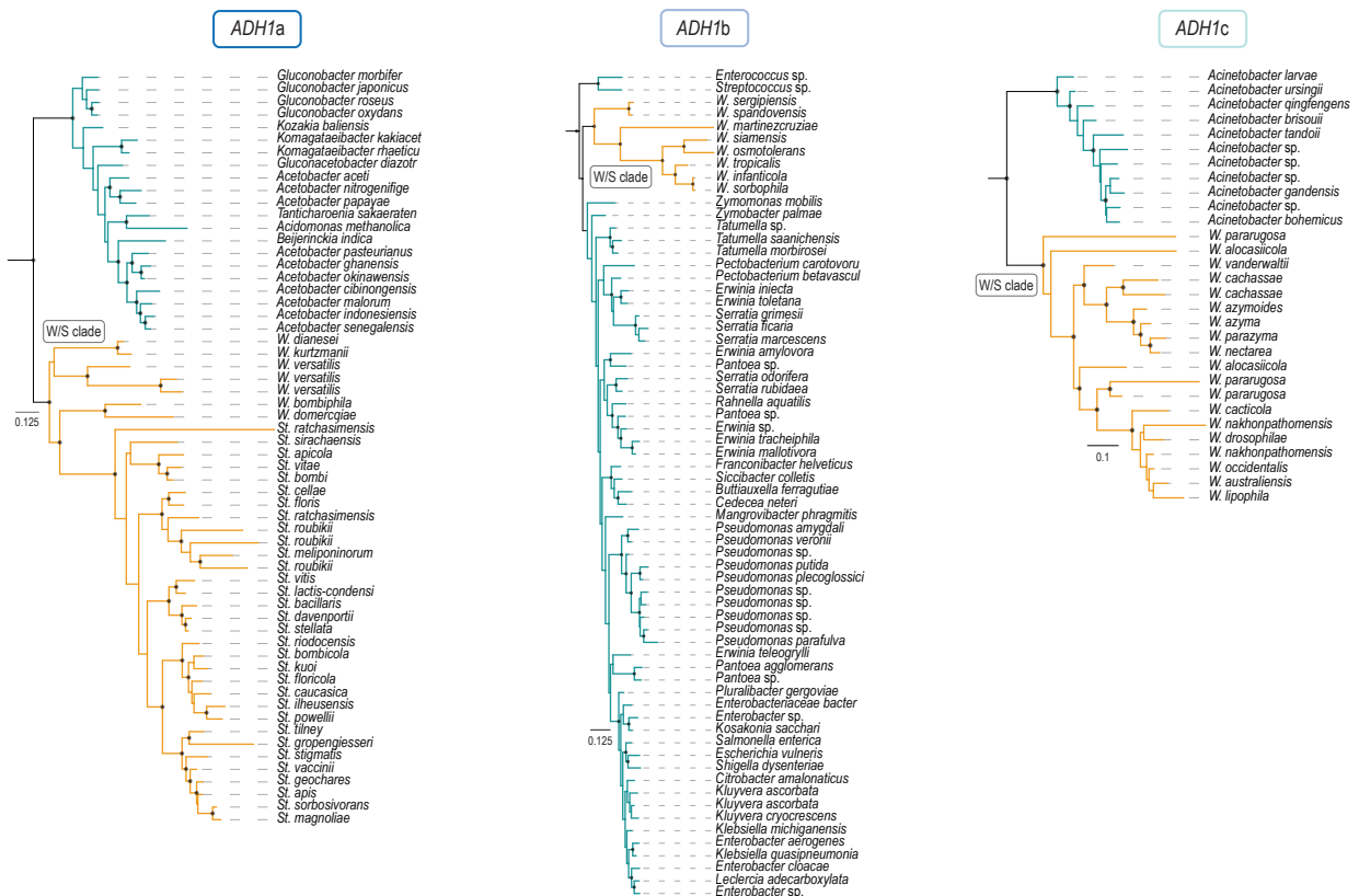
Supplementary Figure S1. Fig. S1. Maximum-likelihood phylogeny of Adh1 proteins. (A) The different lineages are represented by different branch colors (red for Saccharomycotina, light brown for other Fungi (i.e., non-Saccharomycotina), orange for the W/S clade and blue for bacteria). Poorly represented lineages (< 10 sequences) are shown in grey. Branches with bootstrap support higher than 95% are indicated by black dots. (B) Pruned maximum-likelihood phylogenies of Adh1 proteins depicting the phylogenetic relationship between the W/S clade and closest related species.
