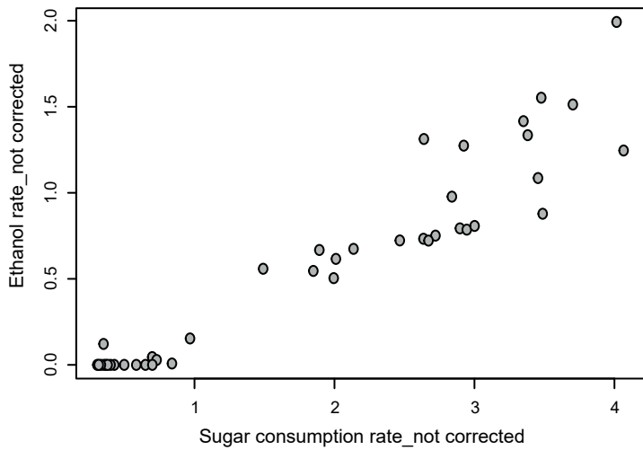
Supplementary Figure S5. Phylogenetic correction of the correlation between sugar consumption rates and fermentation byproducts production rates across the W/S clade. On the left, original values for sugar consumption rates and fermentation byproducts rates (A) or ethanol production rates (B) are shown. On the right, respective PIC (phylogenetic independent contrasts) corrected values are represented.
