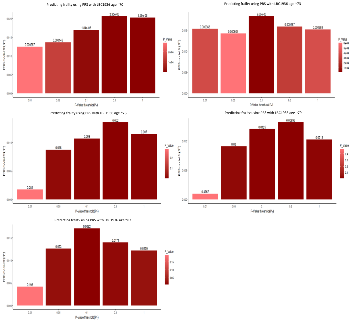
Figure S1. Multiple bar plots, from the multiple regression models, showing the optimal p-value thresholds when predicting frailty using PRS at five time points the LBC1936. The x axis displays the varying different p-value threshold levels. The y axis displays the variance explained by the PGS. The values above the bar are the p-values from the regression output. The darker and taller the bar the stronger the prediction of the frailty PGS.
