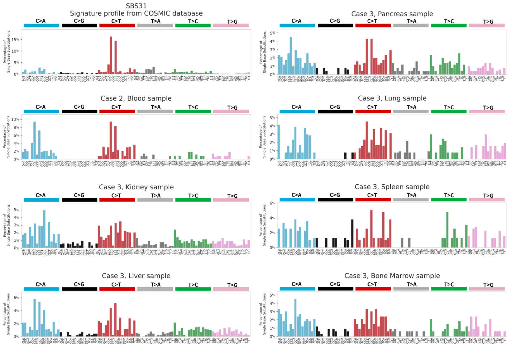
Supplementary Figure 11. Mutational profiles of the samples sequenced with Duplex Sequencing. Upper-left panel is the SBS31 mutational profile from the COSMIC database. Depicted are the profiles from case 2 blood sample and case 3 kidney, liver, pancreas, lung, spleen and bone marrow samples.
