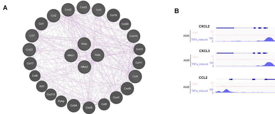
Figure S4. COL1 promotes microglial polarization through the \beta -Integrin/NF- \kappa B signaling. Related to Figure 5.
