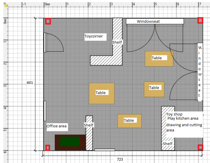
Figure S1. Tracking system: (a) Ubisense tag at approximate scale (1" x 1" x .36") which emits radio signals to (b) sensors arrayed in a classroom space (with dimensions 6.01 m x 7.23 m), where the four red squares in the corners represent the Ubisense radio receivers.
