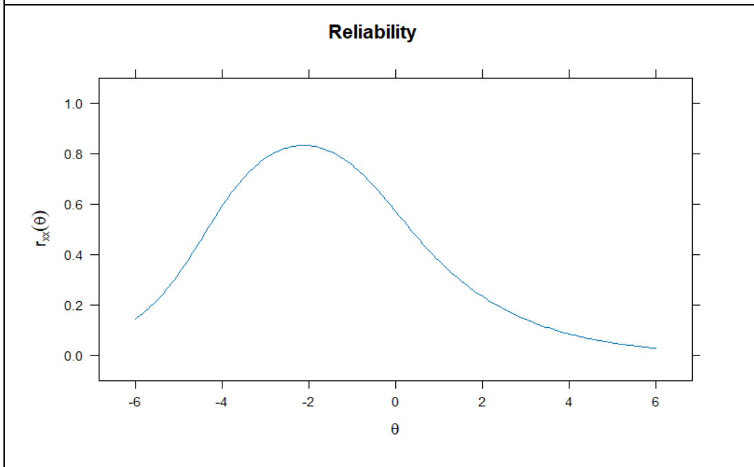
Supplementary Figure 2. Reliability function for the 14-item Attribution Domain plotting Cronbach's alpha coefficient values along the spectrum of possible scores.
