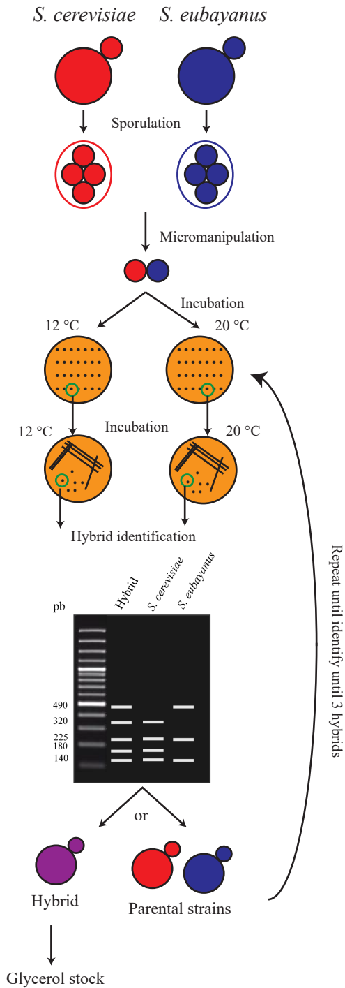
Figure S1. Generation of interspecific S. cerevisiae x S. eubayanus hybrids. Experimental procedure designed to generate and identify interspecific hybrids at two different temperatures (12 and 20°C).
