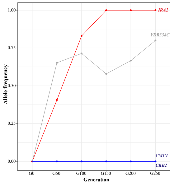
Figure S8. Dynamics of molecular evolution. Allele frequencies over time in H3-4 and H4-1 line evolved in T medium. In red and blue are highlighted SNPs in the genes present in the evolved individuals in the S. cerevisiae and S. eubayanus subgenomes, respectively.
