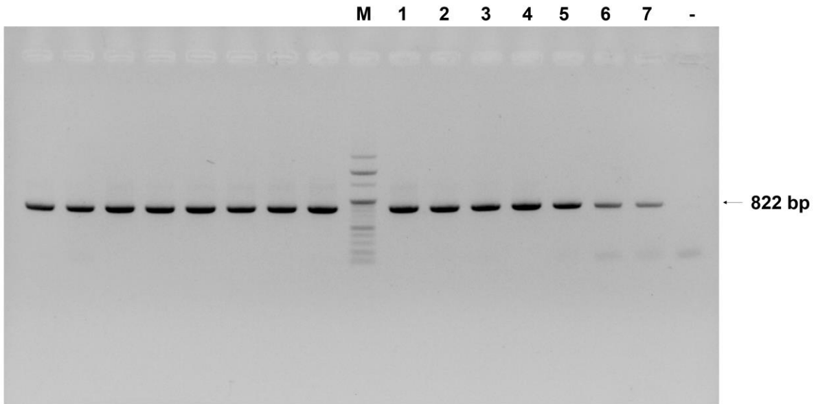
Supplementary Figure 2. Original gel used to prepare Figure 2a. M: 100-bp DNA ladder (Enzynomics, Daejeon, ROK); lanes 1 to 7: PCR performed with DNA template of honeybee samples; (-): PCR without DNA template. AmFV, Apis mellifera filamentous virus; PCR, polymerase chain reaction; ROK, Republic of Korea.
