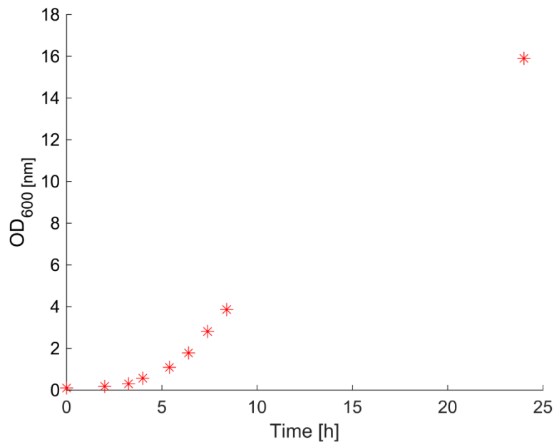
14 Fig. S1 Growth curve of Saccharomyces cerevisiae in YPD medium. Growth conditions: 120 rpm, 15 32°C, pH 6.2
