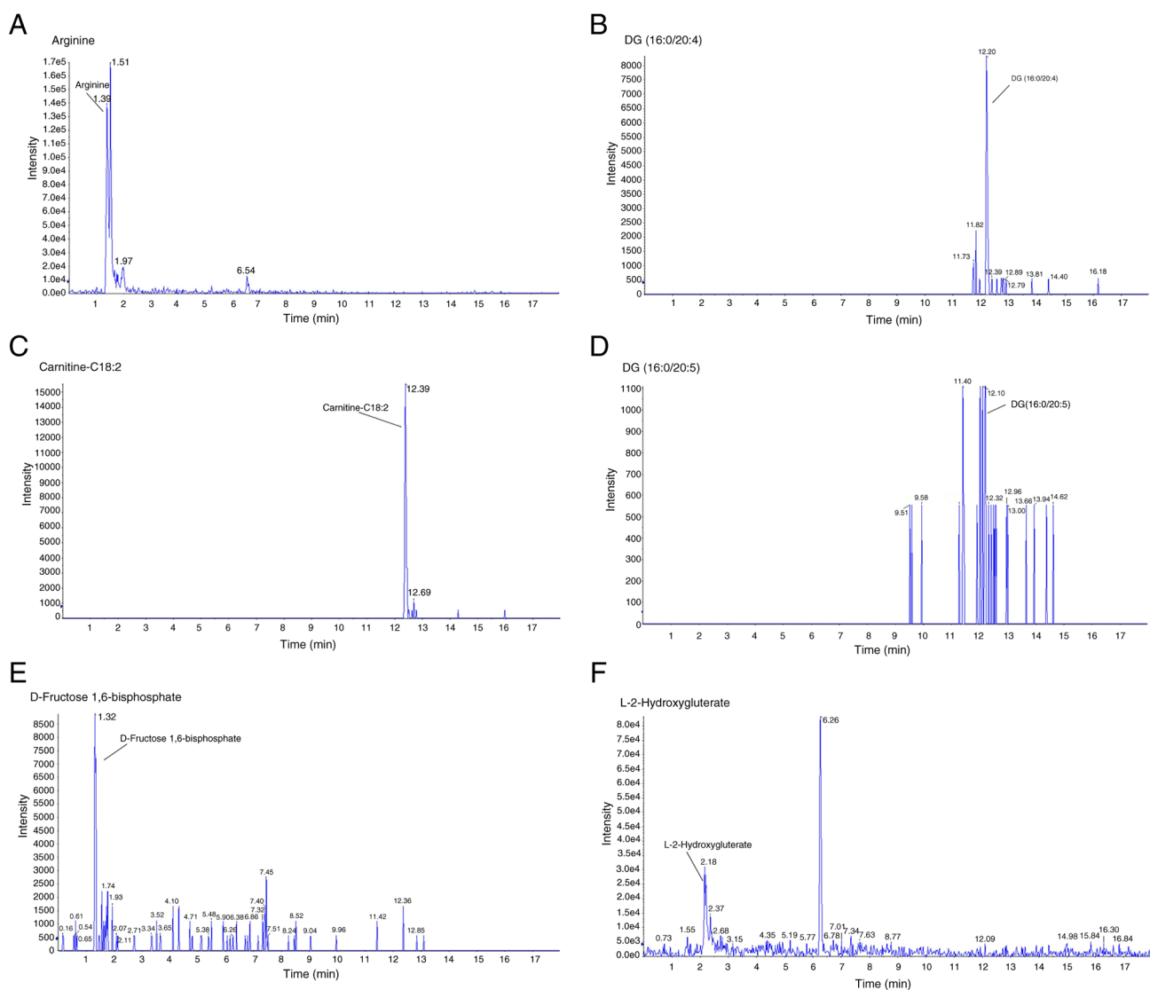
Figure S1. Extracted ion chromatograms of differential metabolites. (A) Arginine, (B) DG (16:0/20:4), (C) carnitine-C18:2, (D) DG (16:0/20:5), (E) D-fructose 1,6-bisphosphate and (F) L-2-hydroxyglutarate. DG, diacylglycerol.
