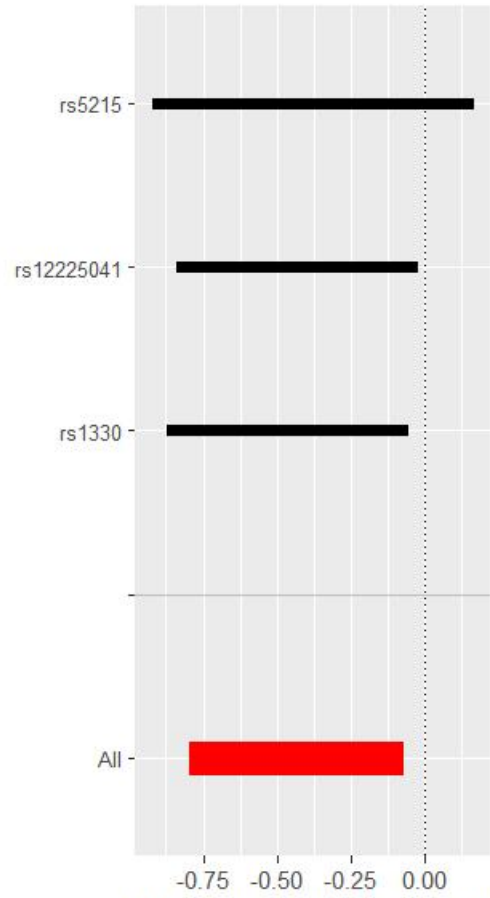
MR leave-one-out sensitivity analysis for els || id:ebi-a-GCST90025986' on 'Gastroesophageal reflux
