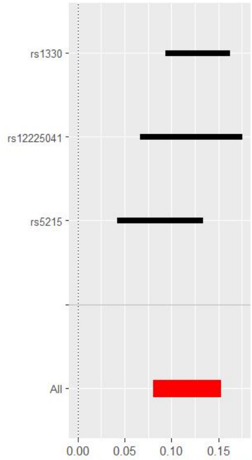
MR leave-one-out sensitivity analysis for || id:ebi-a-GCST90025986 on 'Non-cancer illness code, se
