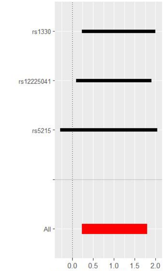
MR leave-one-out sensitivity analysis for lucose levels || id:ebi-a-GCST90025986' on 'Gastric ulcer ||
