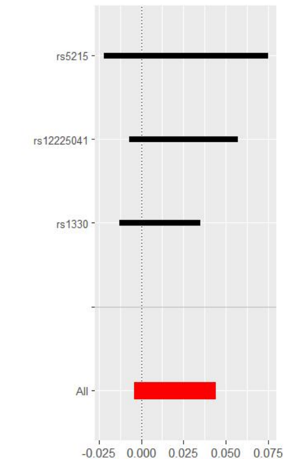
MR leave-one-out sensitivity analysis for d glucose levels || id:ebi-a-GCST90025986 on 'Colorectal c
