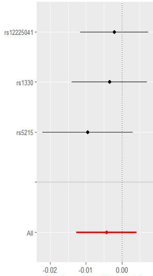
MR leave-one-out sensitivity analysis for s || id:ebi-a-GCST90025986 on 'Non-cancer illness code, self-report
