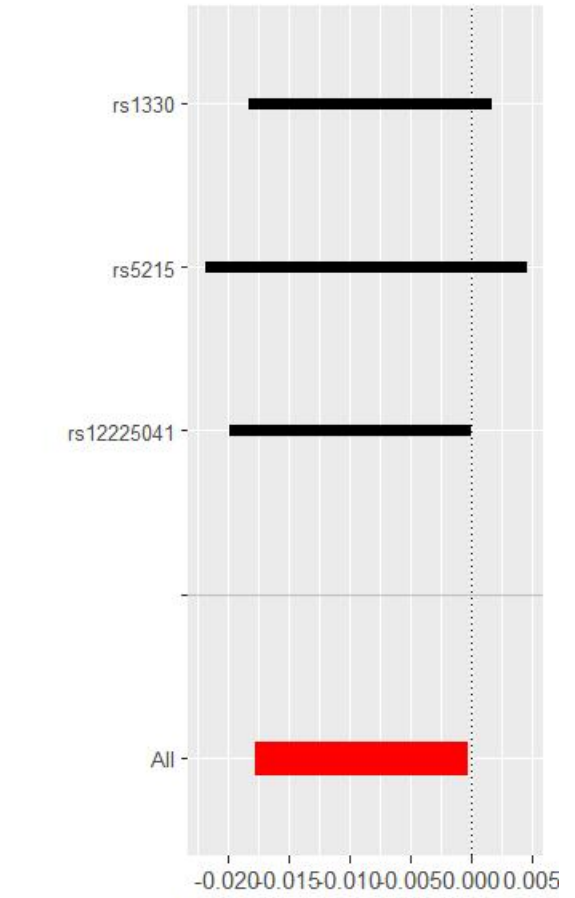
MR leave-one-out sensitivity analysis for bi-a-GCST90025986' on 'Diagnoses - main ICD10: K29.5 C
