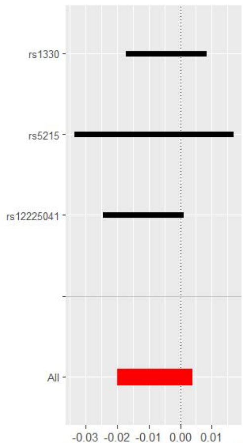
MR leave-one-out sensitivity analysis for d:ebi-a-GCST90025986 on 'Non-cancer illness code, self-re
