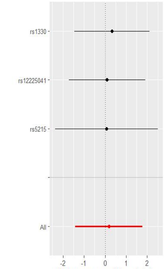
MR leave-one-out sensitivity analysis for ucose levels || id:ebi-a-GCST90025986 on 'Functional dyspepsia || i
