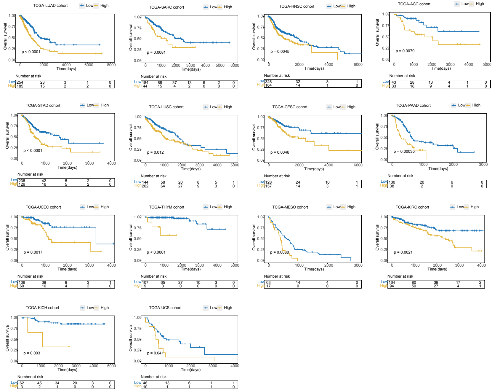
Figure S6 Kaplan-Meier curves show the independent relevance between overall survival time and risk group in 14 TCGA cancer species.
