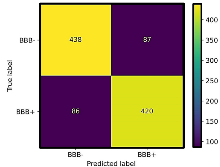
Test Set
