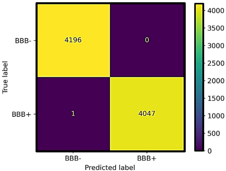
Training Set
