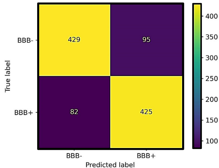
Validation Set
