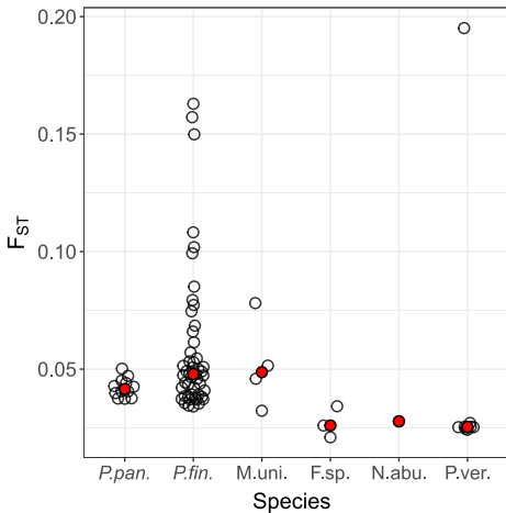
Suppl. Fig. S9.: Population differentiation within the water column. F_{ST} between samples taken from the same habitat at the same time but from different depths. Median values are shown in red.
