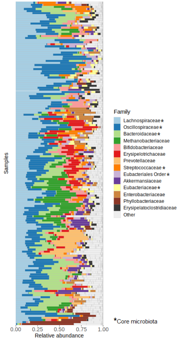
C 16S Family composition
