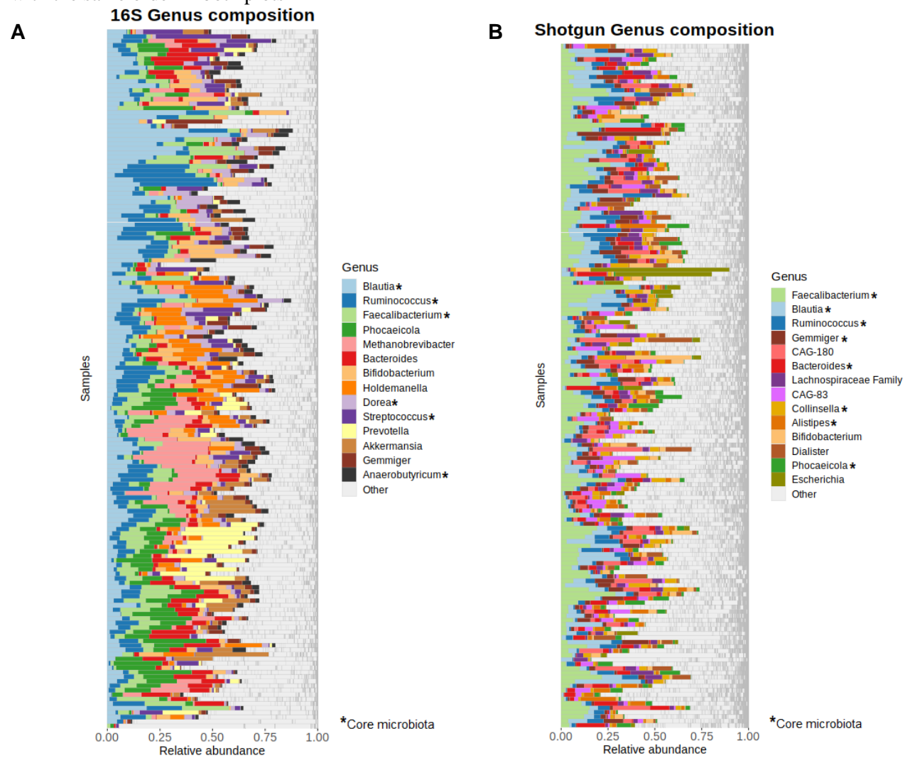
Additional Figure S3. Bar plots of the top 15 most common genera and families in 16S and shotgun abundance data. Each row represents a different sample with the same order in both plots
