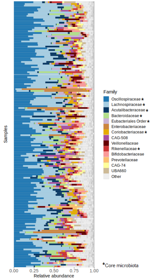
D Shotgun Family composition
