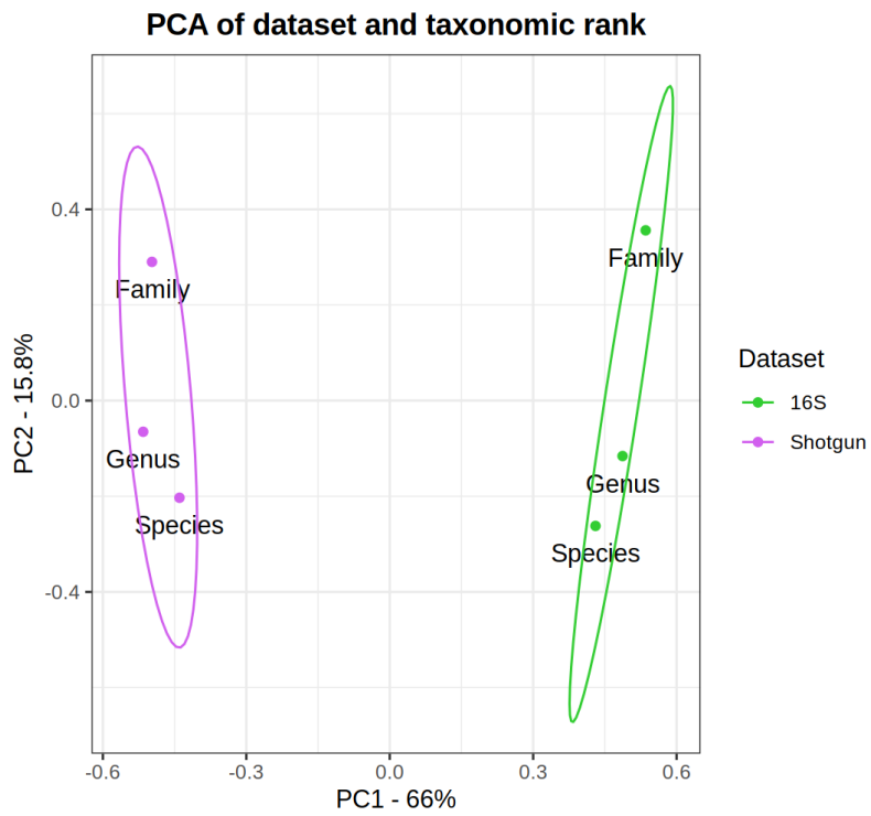
Additional Figure 4 PCA summary of similarities among datasets (shotgun vs 16S in the three taxonomic ranks):
