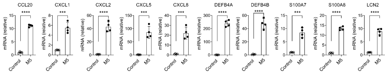
Figure s2. M5 cocktail cytokines induce the upregulation of psoriasis related T cell chemokines, neutrophil chemokines, and antimicrobial peptides in HaCat cells.
