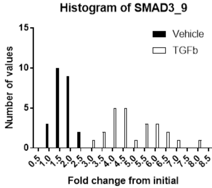
Figure S1: Histogram of raw fold change values from baseline for the SMAD3_9 reporter 4 hours post stimulation with TGF \beta
