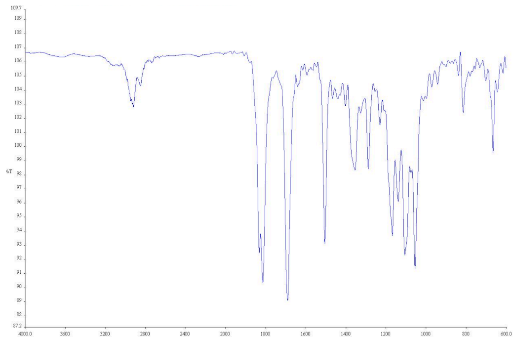
Infrared spectrum (Thin Film, NaCl) of compound 34 .
