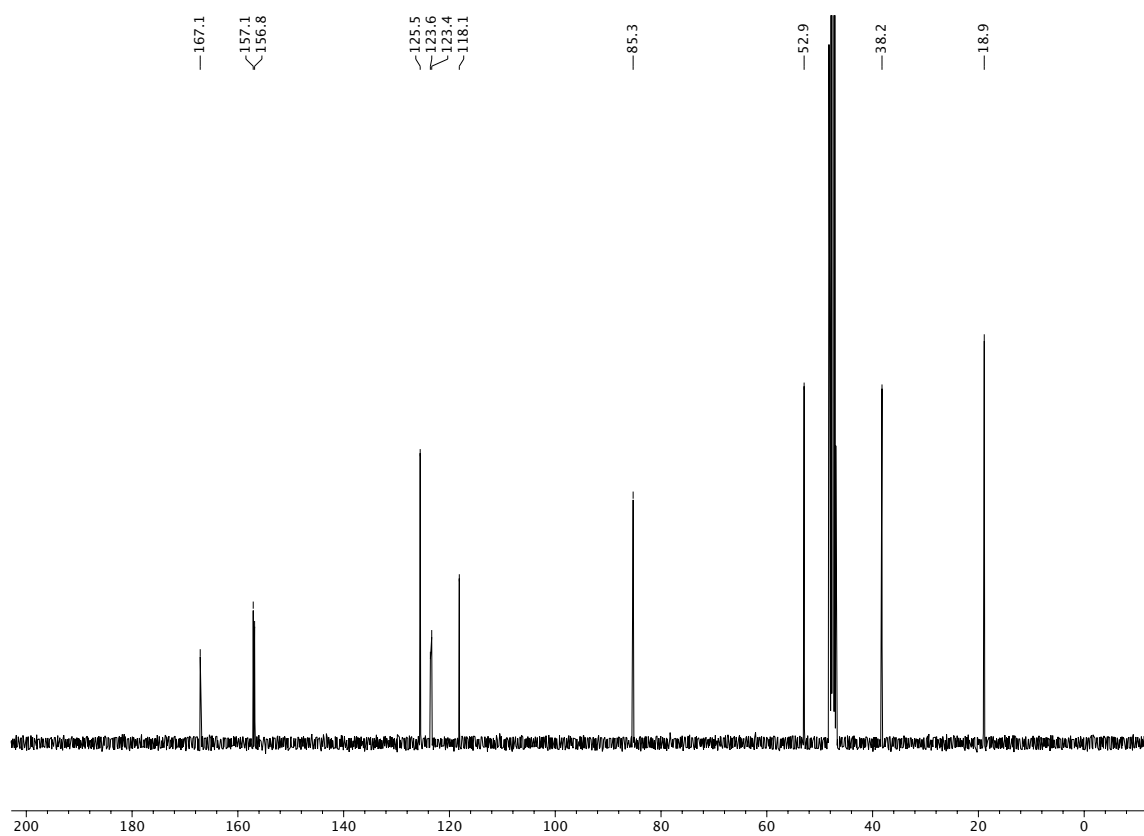
^{13}\text{C} NMR (100 MHz, MeOD) of makaluvamine C ( 23 ).
