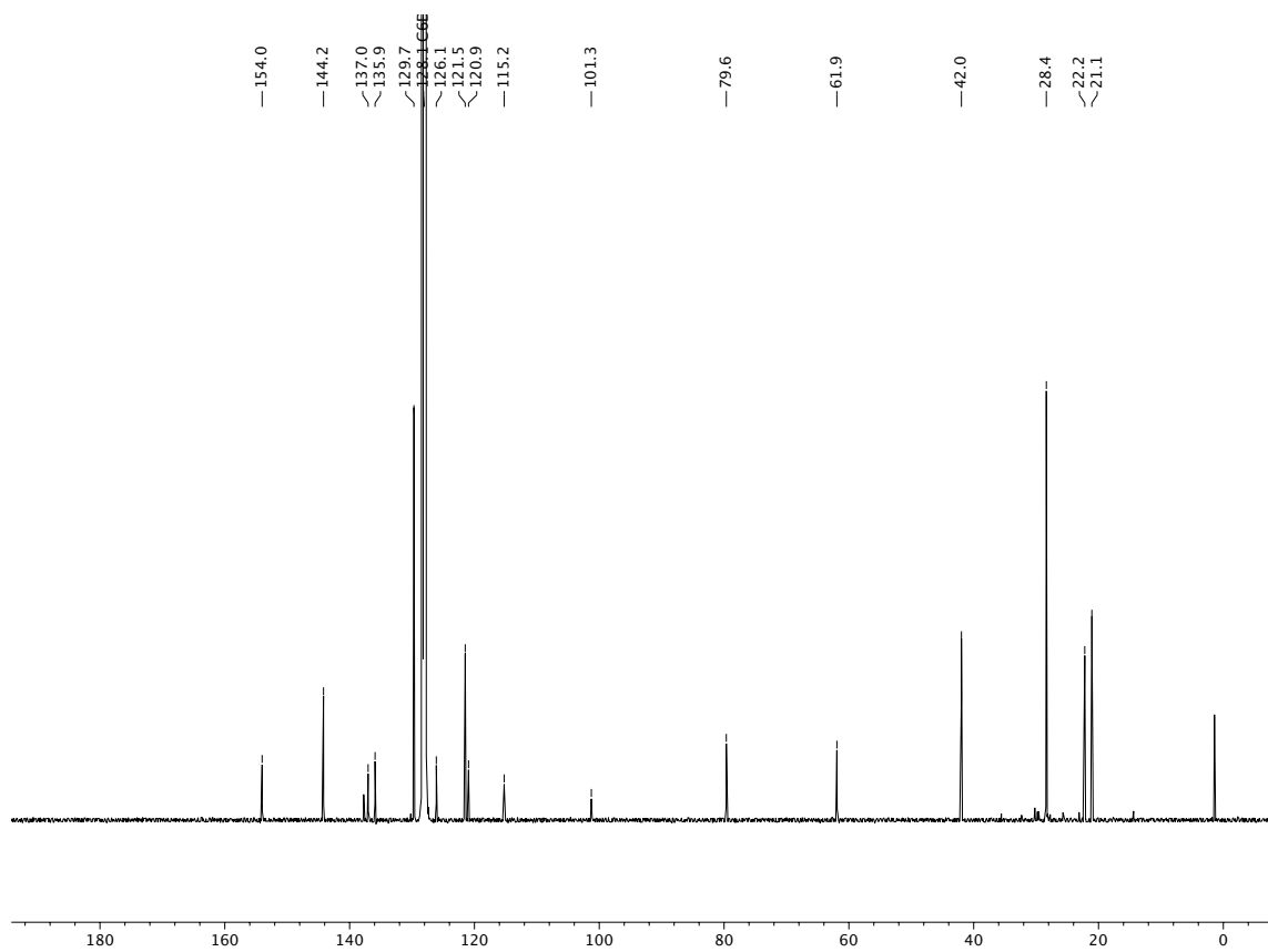
^{13}\text{C} NMR (100 MHz, \text{C}_6\text{D}_6 ) of compound 35 .
