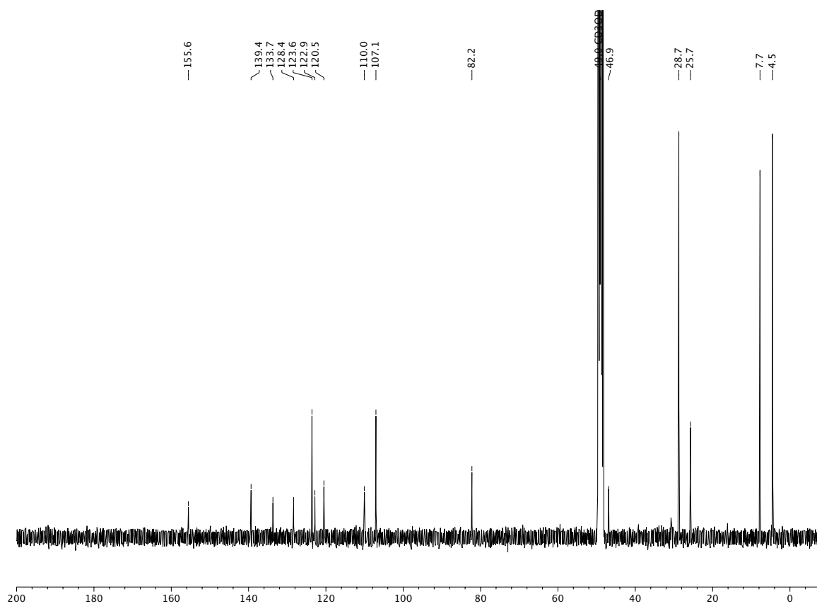
^{13}\text{C} NMR (100 MHz, MeOD) of compound 16 .
