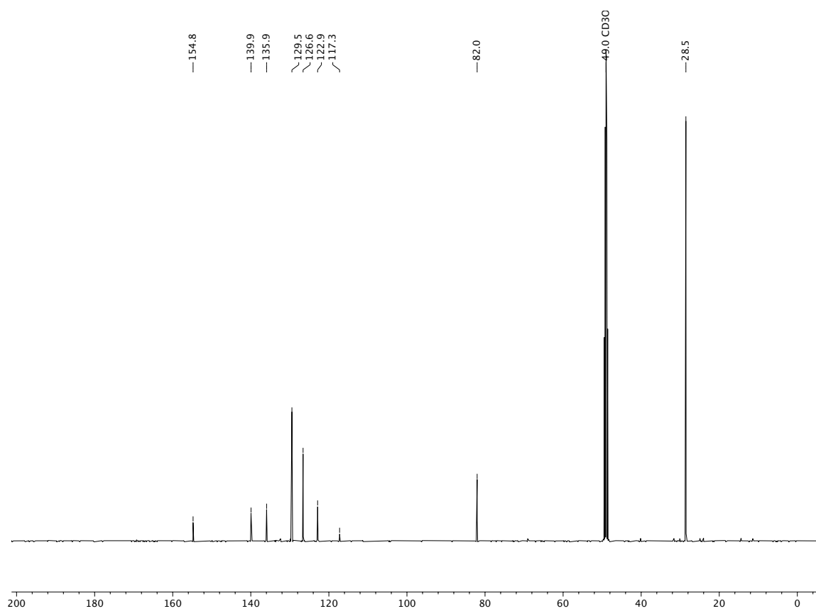
^{13}\text{C} NMR (100 MHz, MeOD) of compound S6 .
