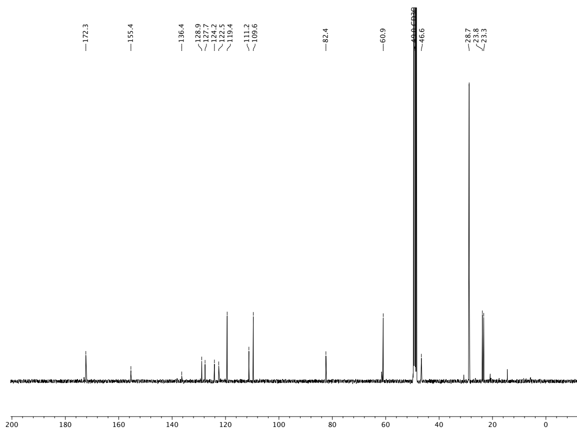
^{13}\text{C} NMR (100 MHz, MeOD) of compound 21 .
