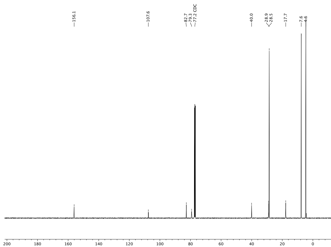
^{13}\text{C} NMR (100 MHz, \text{CDCl}_3 ) of compound S3 .
