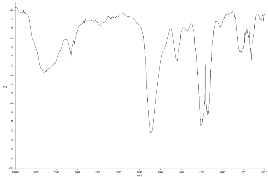
Infrared spectrum (Thin Film, NaCl) of makaluvamine D (29).
