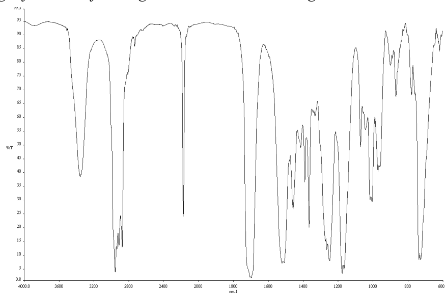
Infrared spectrum (Thin Film, NaCl) of compound 13 .
