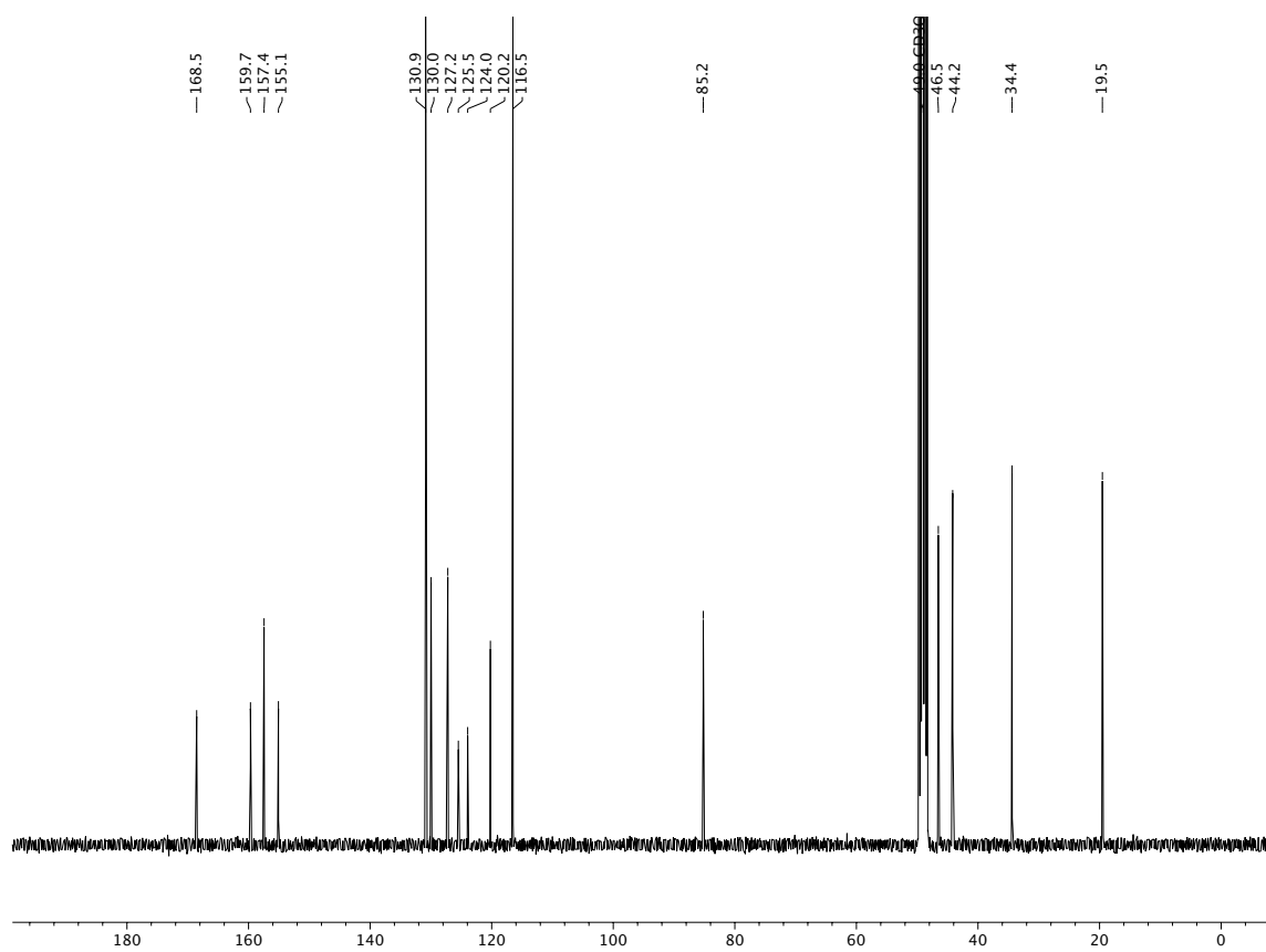
13 C NMR (100 MHz, MeOD) of makaluvamine D (29).
