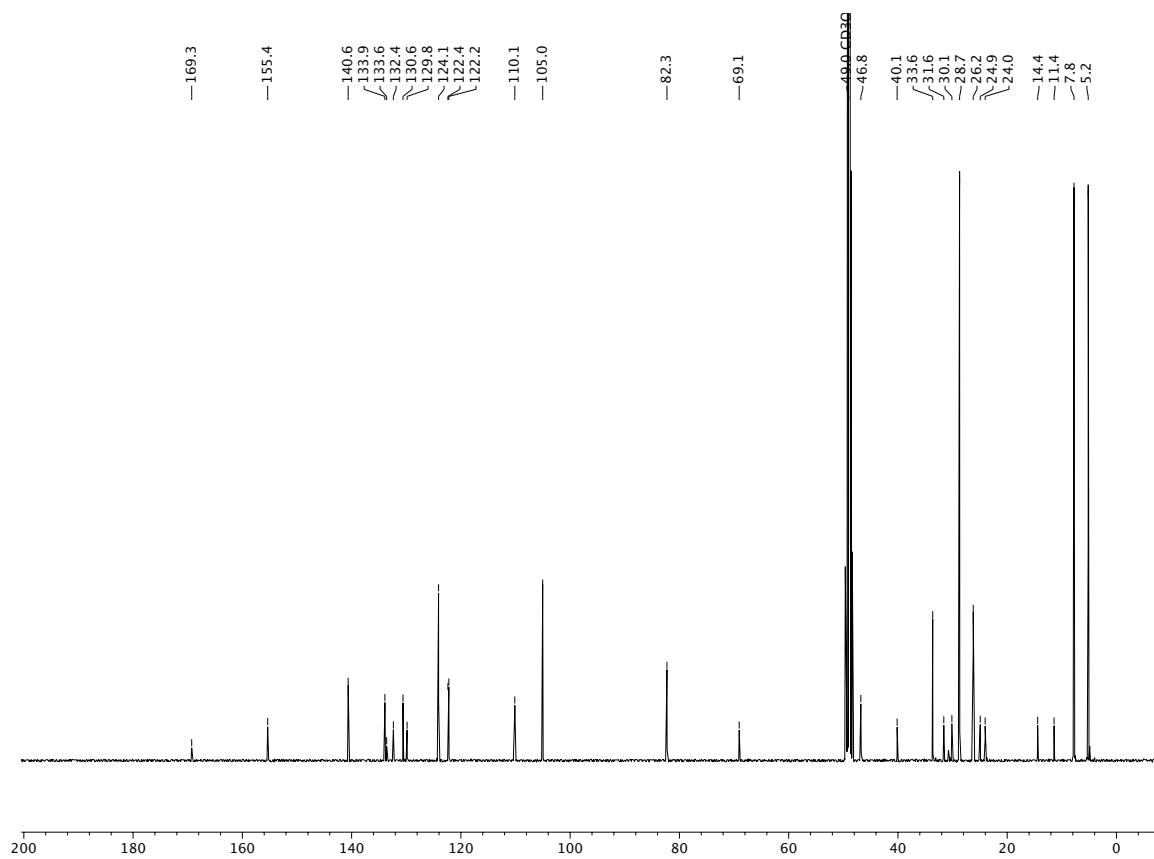
13 C NMR (100 MHz, MeOD) of compound 17 .
