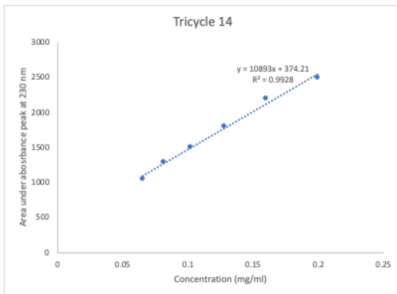
Figure S1. Calibration curve for LC/MS assay for ligand stoichiometry experiments.
