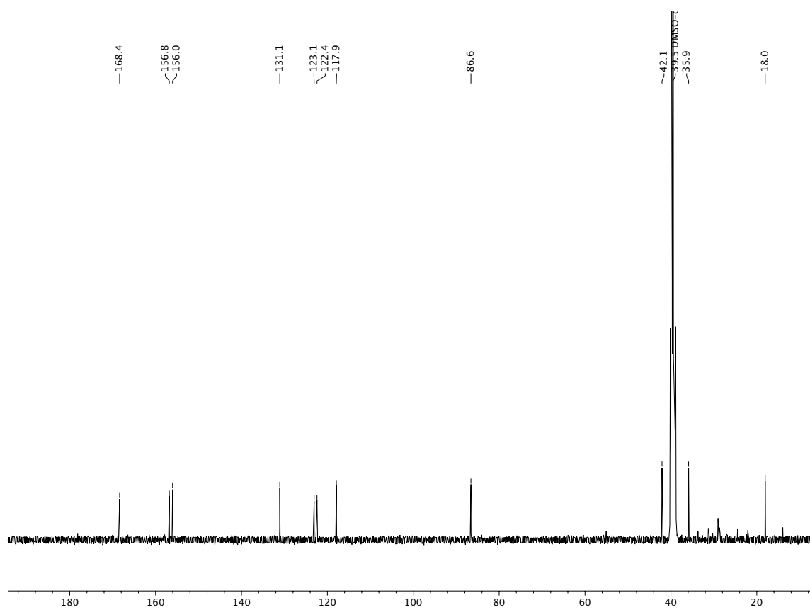
13 C NMR (100 MHz, DMSO-d 6 ) of makaluvamine A ( 26 ).
