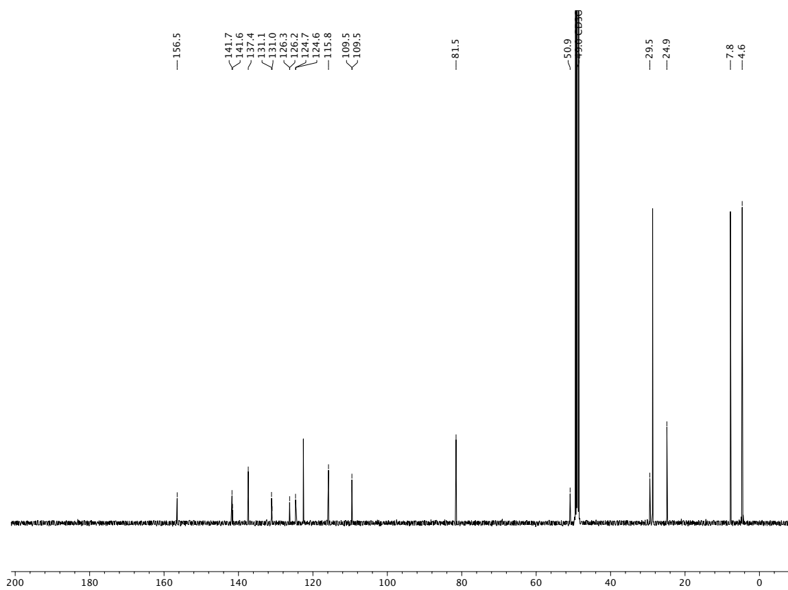
^{13}\text{C} NMR (100 MHz, \text{CD}_3\text{OD} ) of compound 20 .
