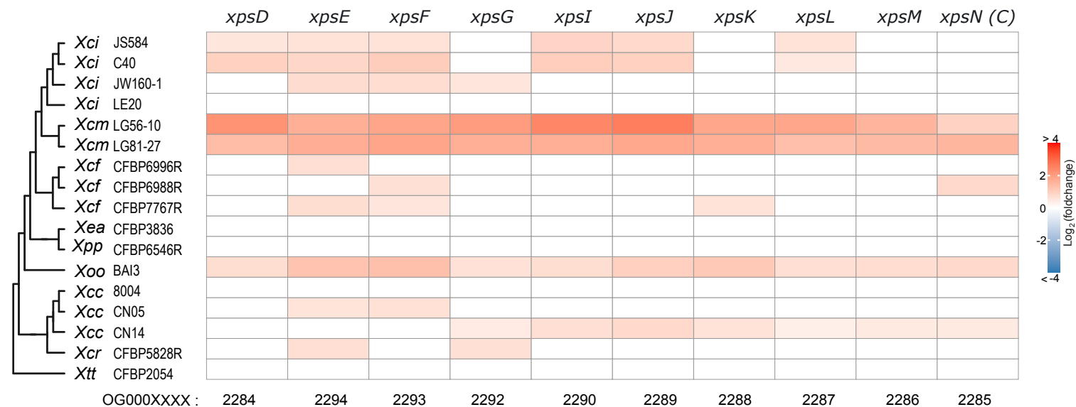
Figure S1: Regulation of orthogroups (OG) encoding different structural components of the T2SS. Only significantly differentially expressed ( \text{AdjPval} < 0.05 ) genes are colored. Orthogroup annotation is given on top of the figure, orthogroup number at bottom of the figure.
