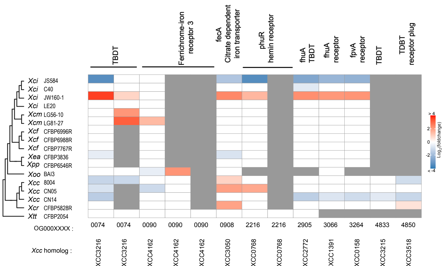
Figure S2: Regulation of orthogroups (OG) encoding genes putatively involved in iron uptake. Only significantly differentially expressed ( \text{AdjPval} < 0.05 ) genes are colored. Orthogroup annotation is given on top of the figure, orthogroup number at bottom of the figure. Genes represented are orthologs of genes identified to be involved in iron uptake in Xcc and are induced upon iron starvation (Blanvillain et al. , 2007).
