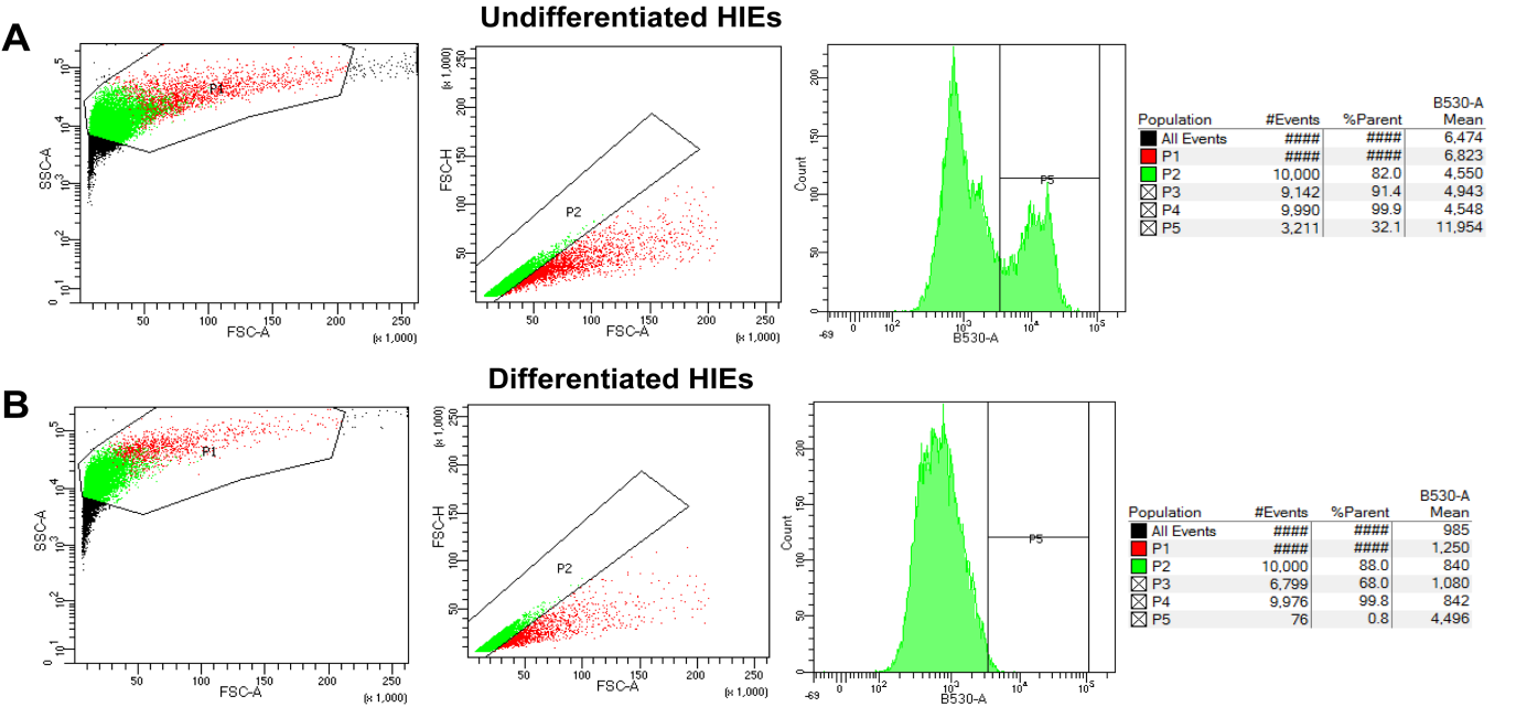
Supplemental Figure 9: Representative EdU gating strategy for undifferentiated (A) and differentiated (B) HIEs
