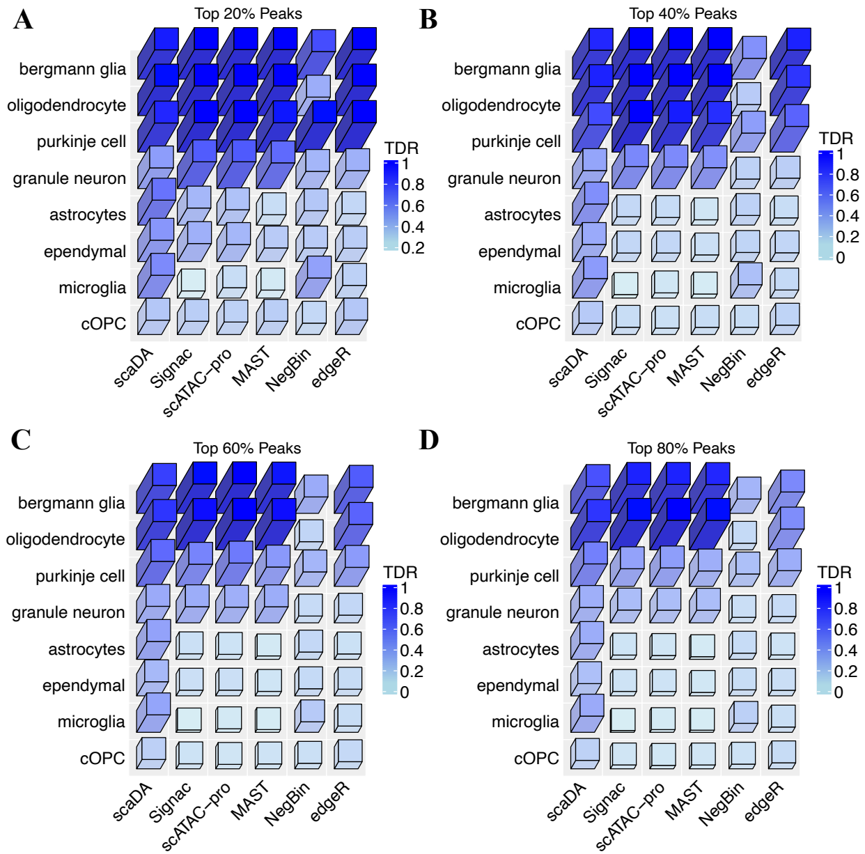
S8 Fig. Human Brain 3K: TDR across 8 cell types for scaDA and published methods at different levels of top percentages (20%, 40%, 60%, 80%)
