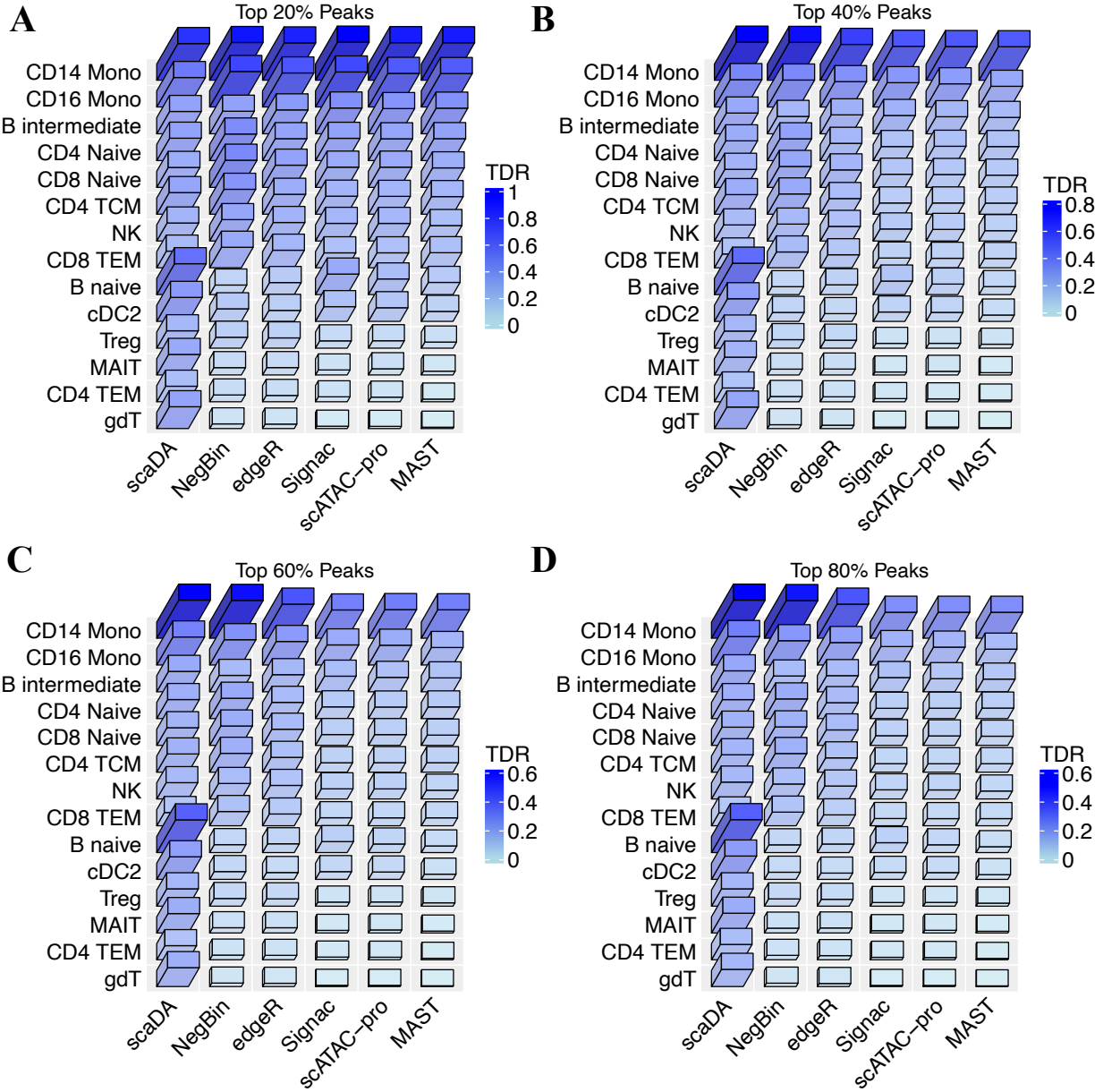
S10 Fig. Human PBMC 10K: TDR across 14 cell types for scaDA and published methods at different levels of top percentages (20%, 40%, 60%, 80%)
