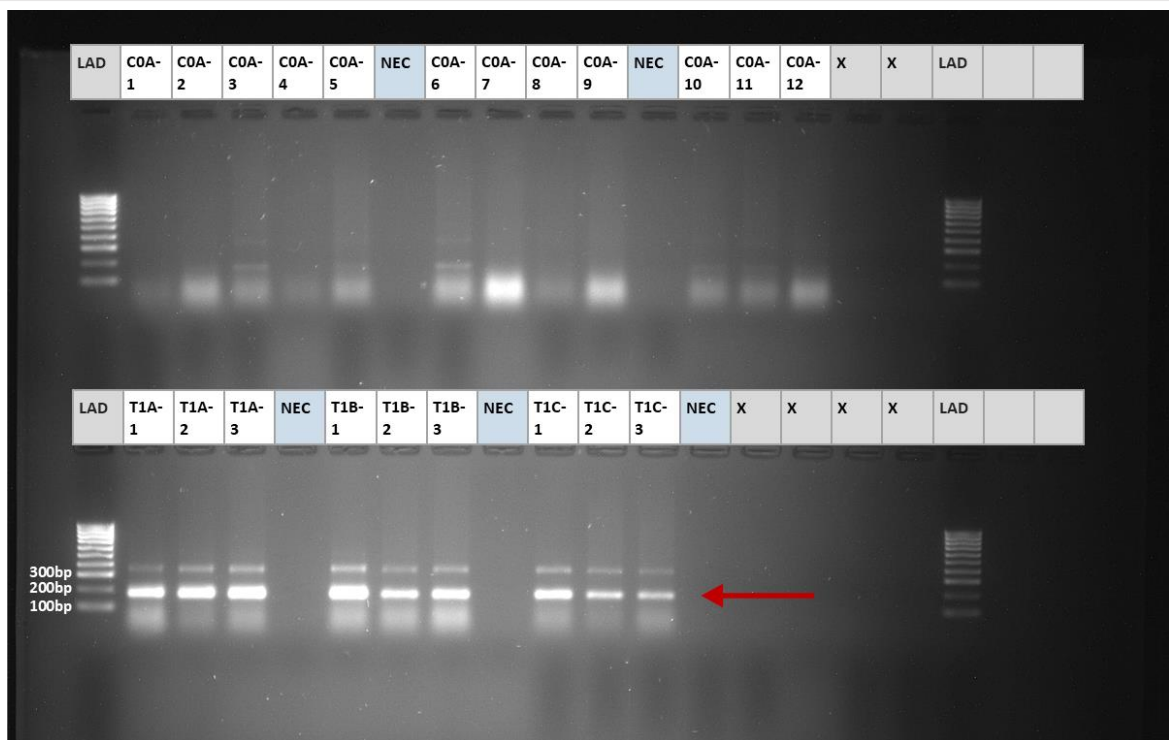
S2 Fig: Gel electrophoresis image from TBR-PCR screening of UFs in C0-A control trap (top row) and naïve flies in T1 control traps (bottom row). Red arrow indicates target 173bp TBR product. NEC = negative extraction control. LAD = 100bp ladder.
