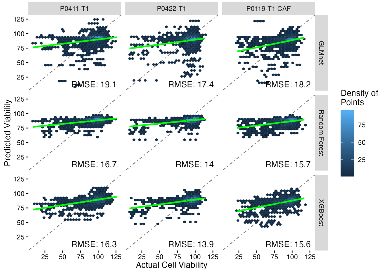
Supplemental Figure 1. Regression models were ineffective at predicting cell viability. The results of the RMSE optimized regression models shown as hex binned heatmaps. Each column shows the optimized results for each cell line, while the rows show the type of model. The dot-dash lines show where a perfect set of predictions would appear, while the green lines show the linear best fit through the presented data points. The RMSE value is also presented in the lower corner of each plot.
