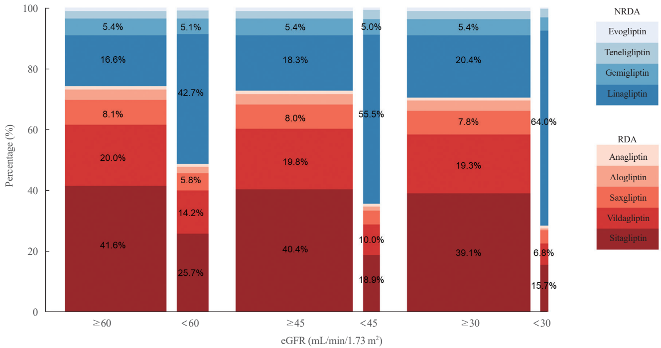
Supplemental Fig. S1. Prescription patterns of renal dose-adjusted (RDA) and non-renal dose-adjusted (NRDA) dipeptidyl peptidase-4 (DPP4) inhibitors according to kidney function. Each bar stacked to represent prescription rates for specific DPP4 inhibitors according to the estimated glomerular filtration rate (eGFR) cutoff values of 60 (left), 45 (middle), and 30 mL/min/1.73 m 2 (right). RDA DPP4 inhibitors are colored in reds and NRDA DPP4 inhibitors in blues. The widths of the columns are proportional to the number of patients in each eGFR group.
