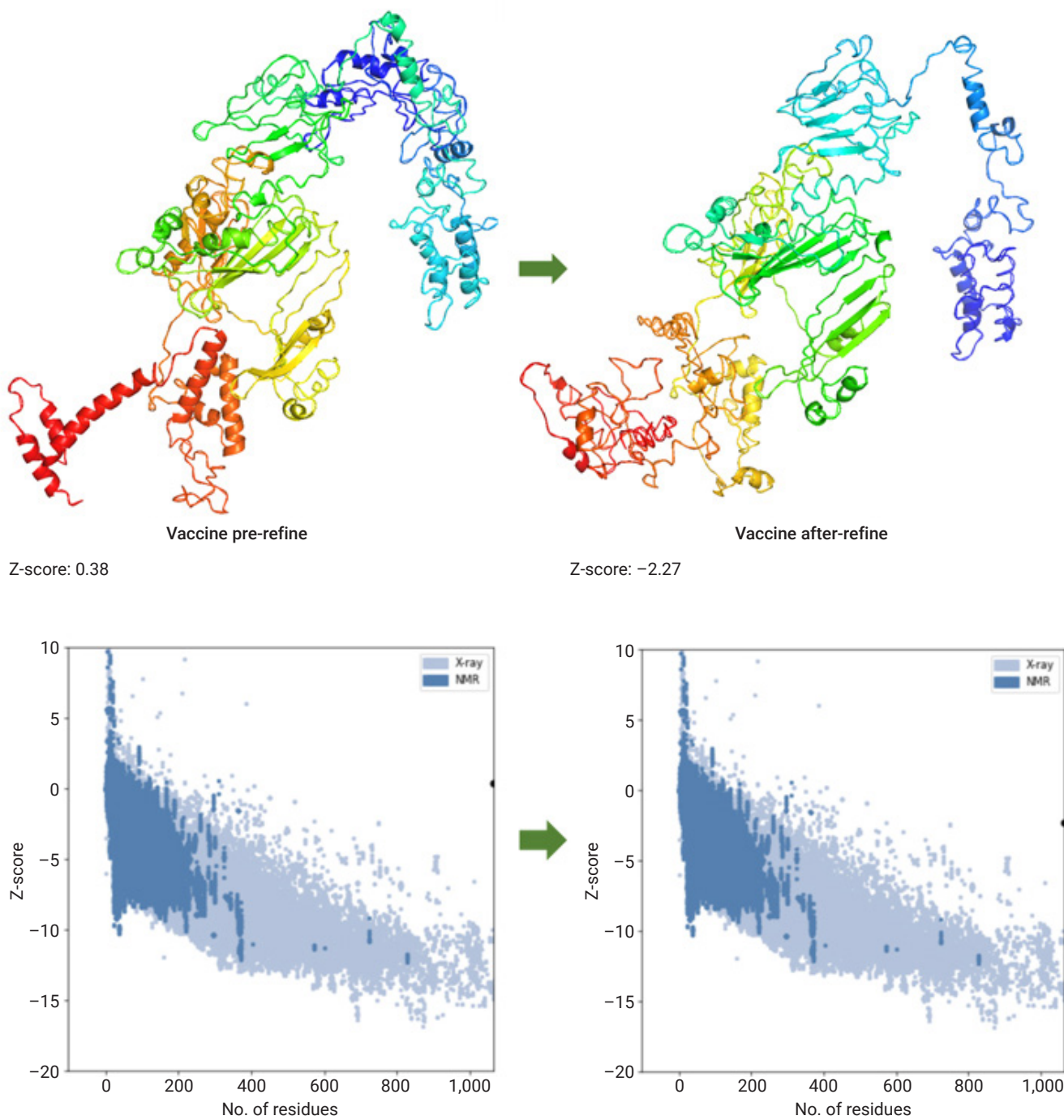
Figure S2. Visualization and Z-score of multi-epitope vaccine constructed before and after refine. NMR, nuclear magnetic resonance.
