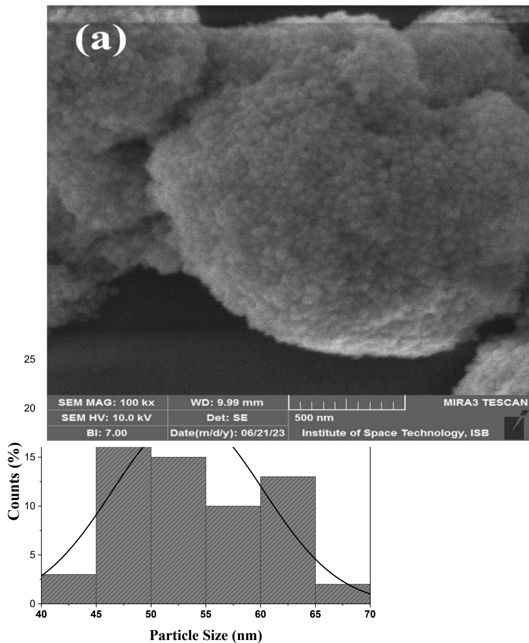
Fig.: SEM image of AgNPs (a), Histogram of AgNPs size (b) and elemental analysis of AgNPs through EDX (c).
