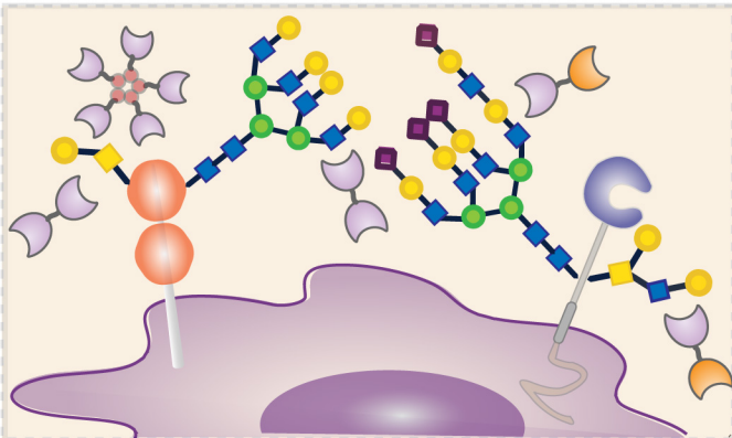
Galectin-glycan interaction
