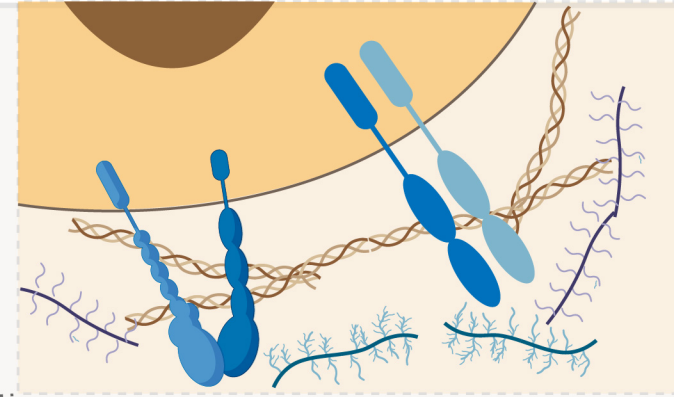
ECM-receptor interaction
