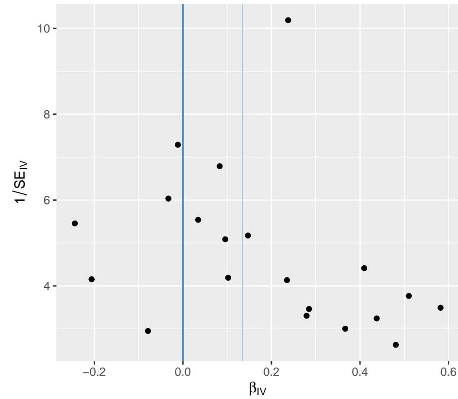
Funnel plot for F10 on BD I
