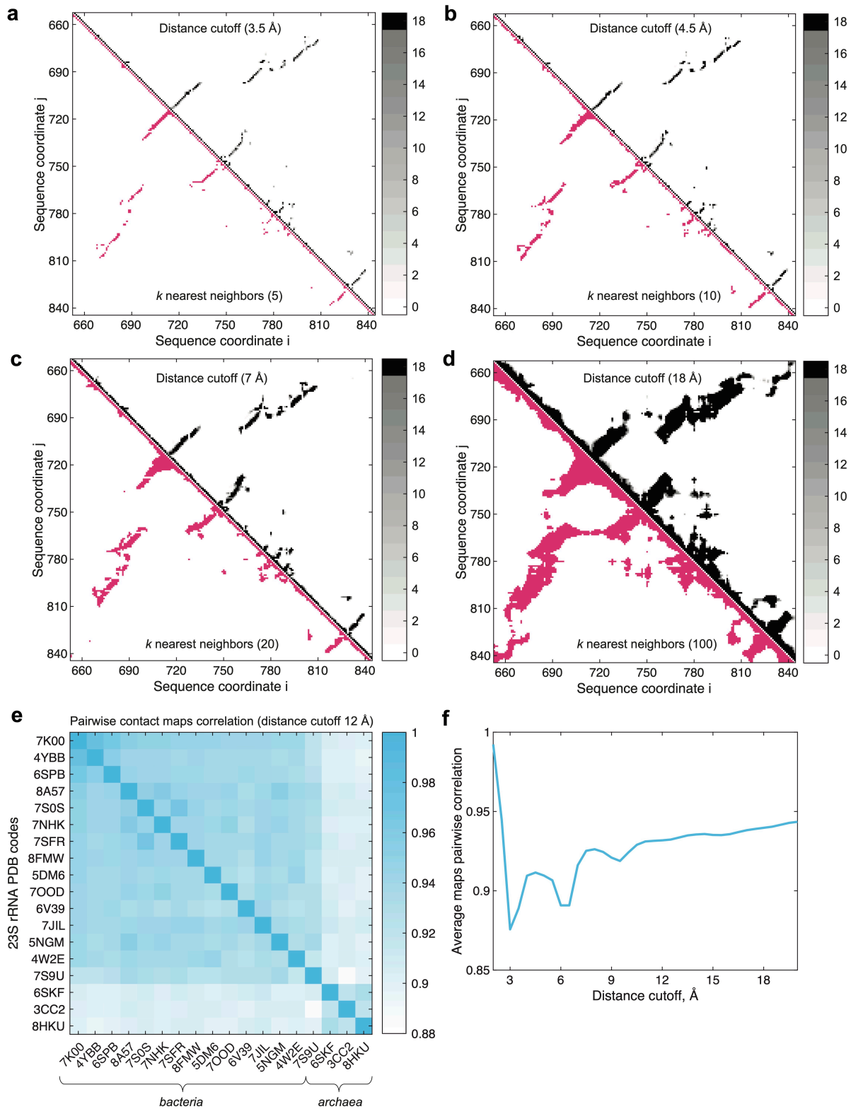
Extended Data Fig. 4: Contact maps and comparisons of high-resolution bacterial and archaeal 50S subunit structures. a-d. Comparison of contact maps generated for
