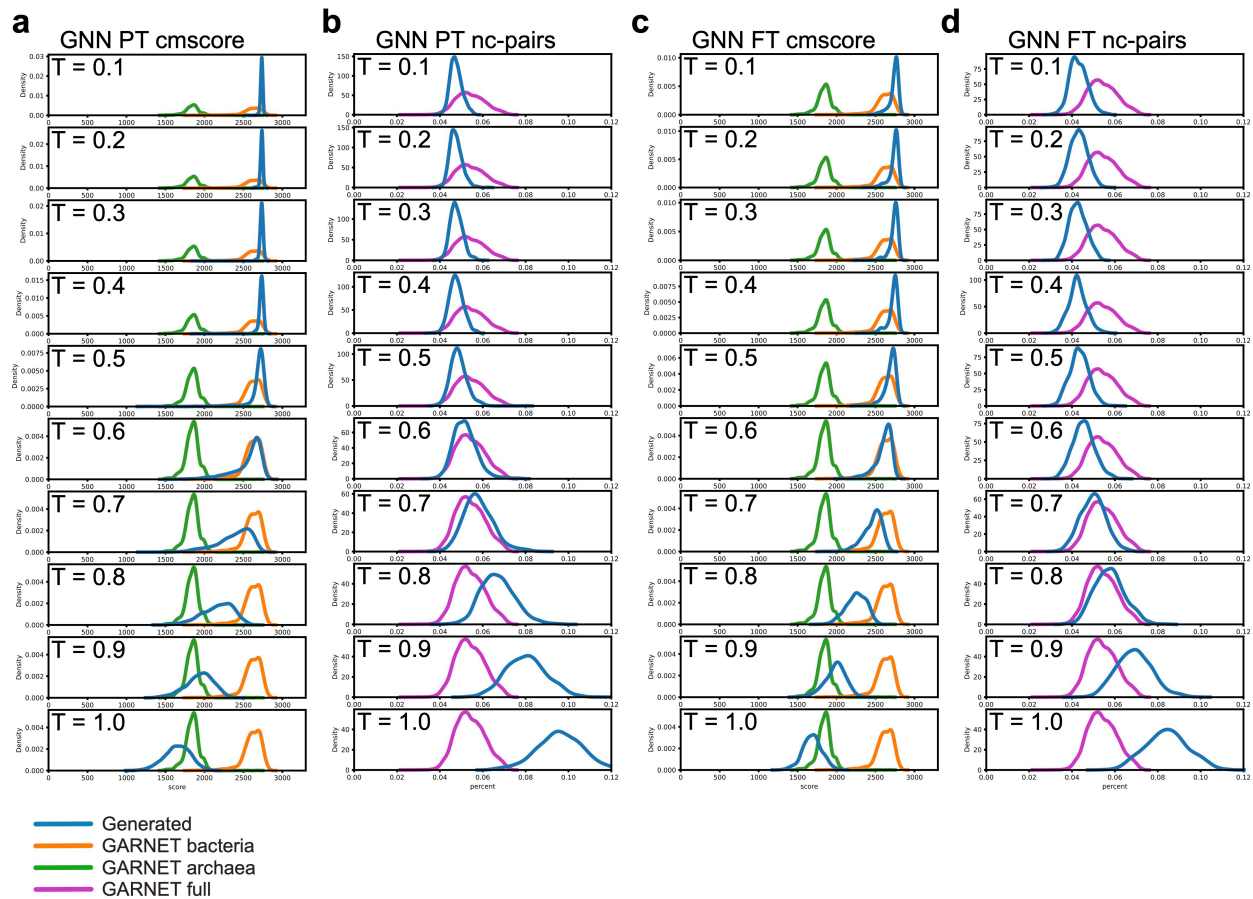
Extended Data Fig. 5: Properties of RNA sequences generated from the 23S rRNA GNN model. a. Cmscore for sequences generated from the pretrained GNN model at temperatures ranging from 0.1 to 1.0. b. Fraction of mismatched nucleotides of sequences generated from the pretrained GNN model relative to RF02541 at temperatures ranging from 0.1 to 1.0. c. Cmscore for sequences generated from the finetuned GNN model at temperatures ranging from 0.1 to 1.0. d. Fraction of mismatched nucleotides of sequences generated from the finetuned GNN model relative to RF02541 at temperatures ranging from 0.1 to 1.0.
