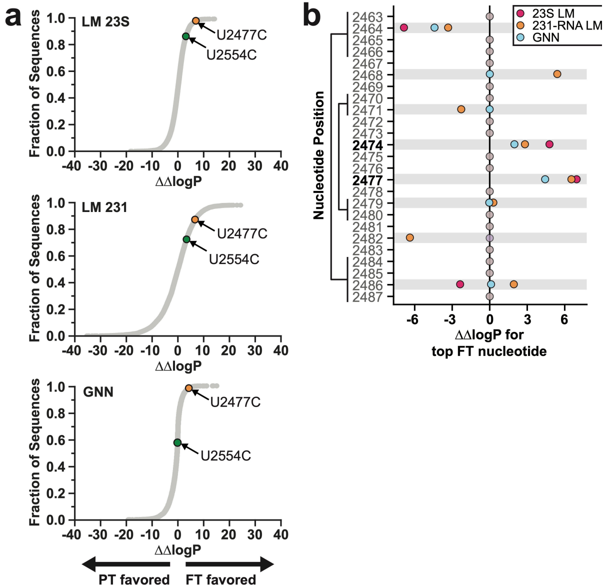
Extended Data Fig. 11: Analysis of \Delta\Delta\log P values for mutations in helix H89. a. Cumulative plots of \Delta\Delta\log P of all single mutations to the E. coli 23S rRNA for each model. Each point represents the probability of generating a single nucleotide mutant E. coli 23S sequence from the FT model relative to the PT model, normalized to that of the WT sequence. Two mutations, U2477C and U2554C, are denoted in orange and green, respectively. b. Analysis of helix 89 for candidate thermostabilizing mutations. For each position, the most frequent nucleotide in FT generated sequences (top FT nucleotide) is grafted into the E. coli 23S rRNA sequence and used to calculate \Delta\Delta\log P(\text{FT-PT}) for the 23S LM, 231-RNA LM, and GNN models. Positions where the top FT nucleotide differs
