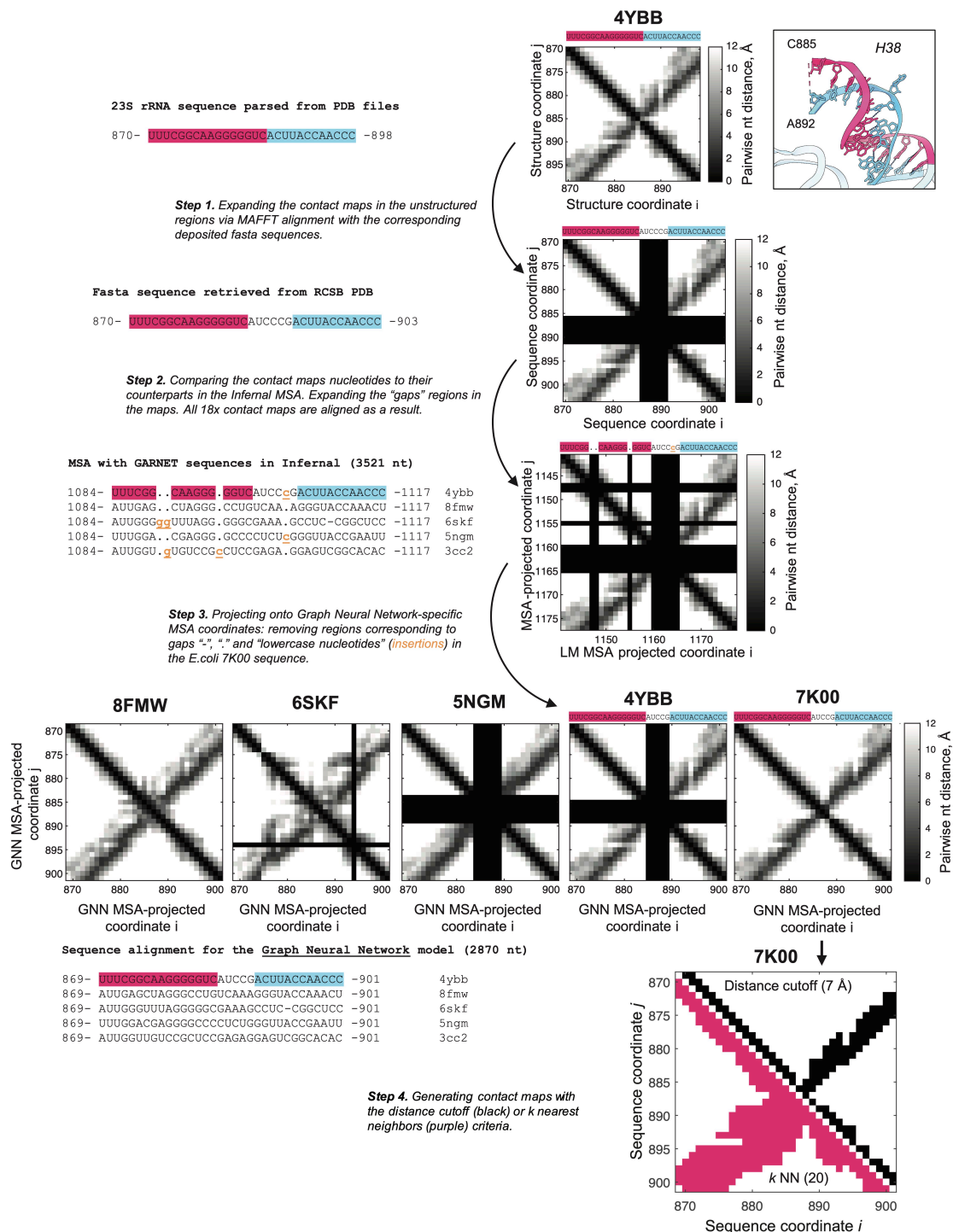
Extended Data Fig. 3: Schematic of MSA-informed alignment of distance matrices from ribosomal structures and generation of contact maps. The initial unaligned pairwise nucleotide distance matrices were generated from 23S rRNA structures in the
