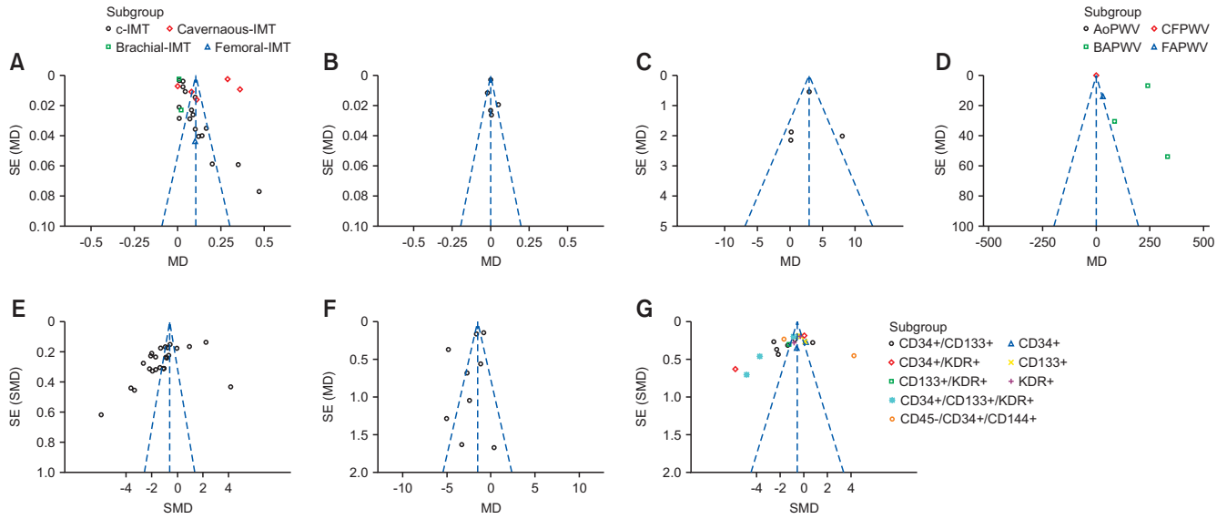
Supplement Fig. 2. Funnel plots of the meta-analysis between erectile dysfunction (ED) and IMT (A), ABI (B), AI (C), PWV (D), FMD (E), NMD (F), and EPC (G). ABI: ankle-brachial index, AI: augmentation index, PWV: pulse wave velocity, FMD: flow-mediated dilation, NMD: nitrate-mediated dilation, EPC: endothelial progenitor cell.
