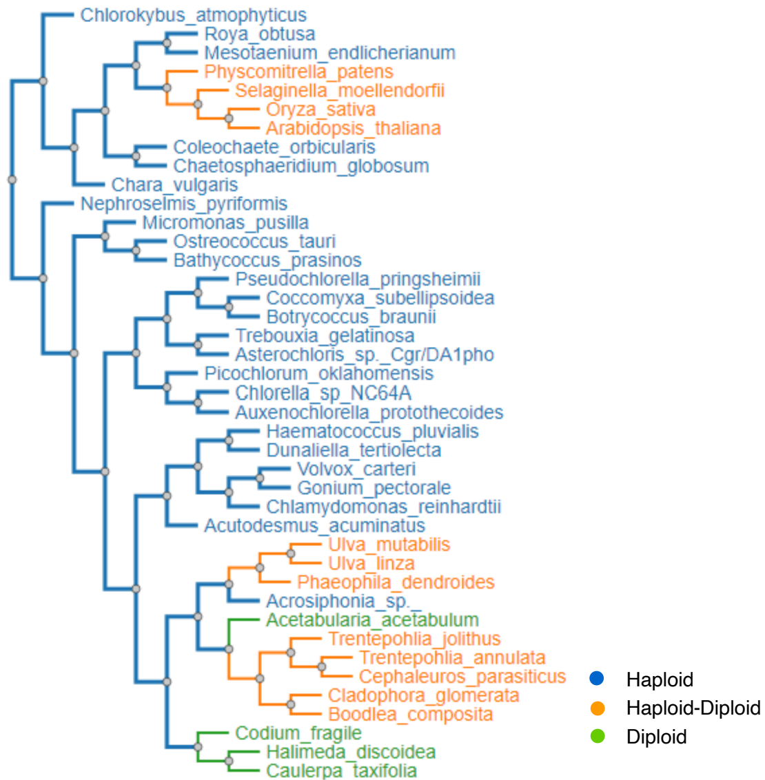
Supplemental Figure S10: Green Algal Phylogeny of liberal dataset showing the trait categories (haploid, haploid-diploid and diploid) for Life cycle based model [M2]. The molecular evolutionary traits: omega ( dN/dS ), non-synonymous ( dN ) and synonymous ( dS ) were obtained for each of the three categories by allowing three different selection pattern corresponding to the trait categories.
