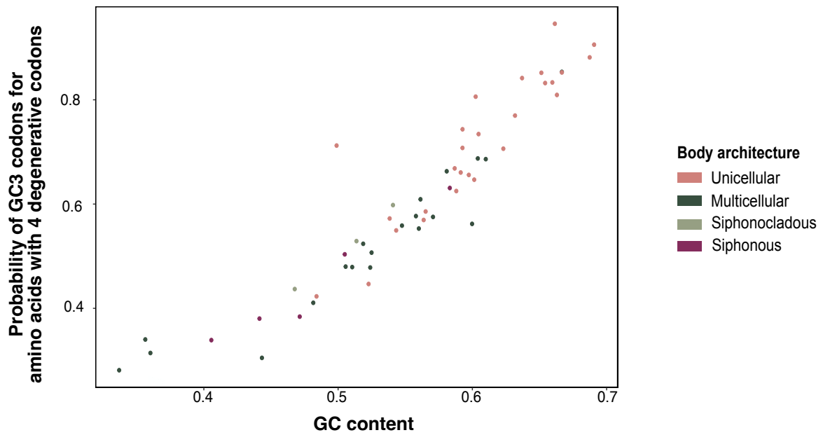
Supplemental Figure S3: Plot showing the correlation between the probability of GC3 codons for amino acids with 4 degenerative codons and GC content. The linear correlation between the probability of GC3 codons for amino acids with 4 degenerative codons and GC content suggests that GC composition is major factor driving usage of these codons.
