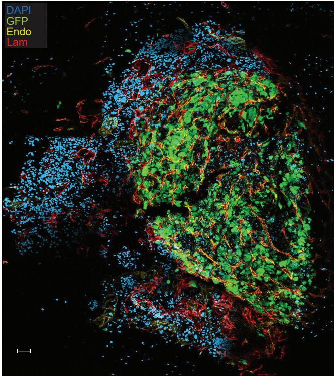
Cabozantinib
