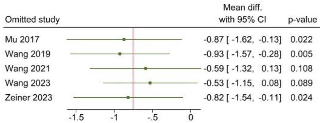
Supplementary Fig. 4. Forest plot for sensitivity analysis of postoperative pain.
