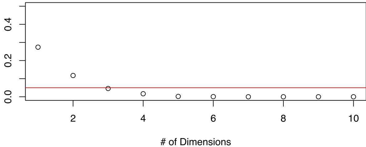
NMDS stress plot
