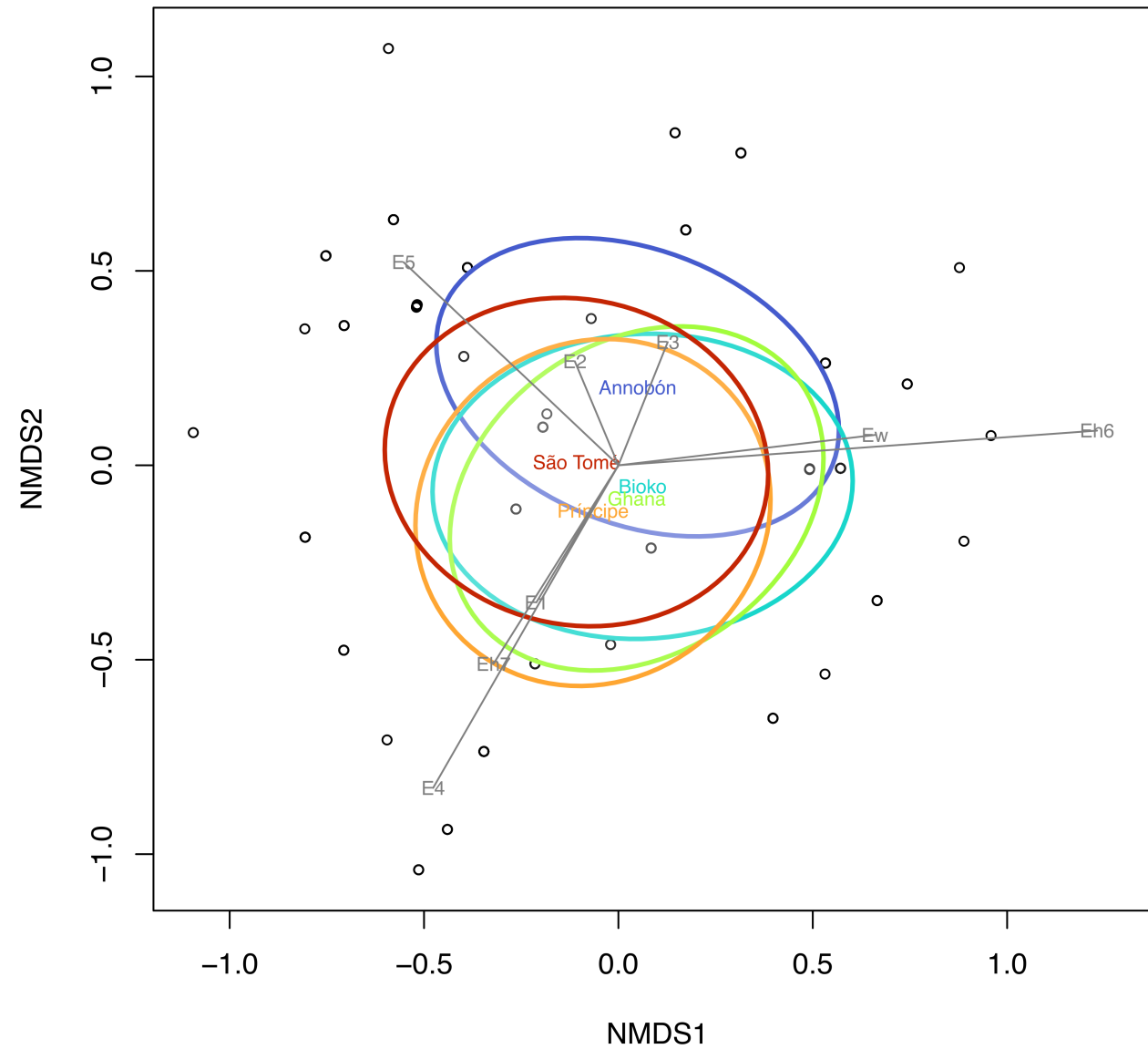
NMDS ordination
