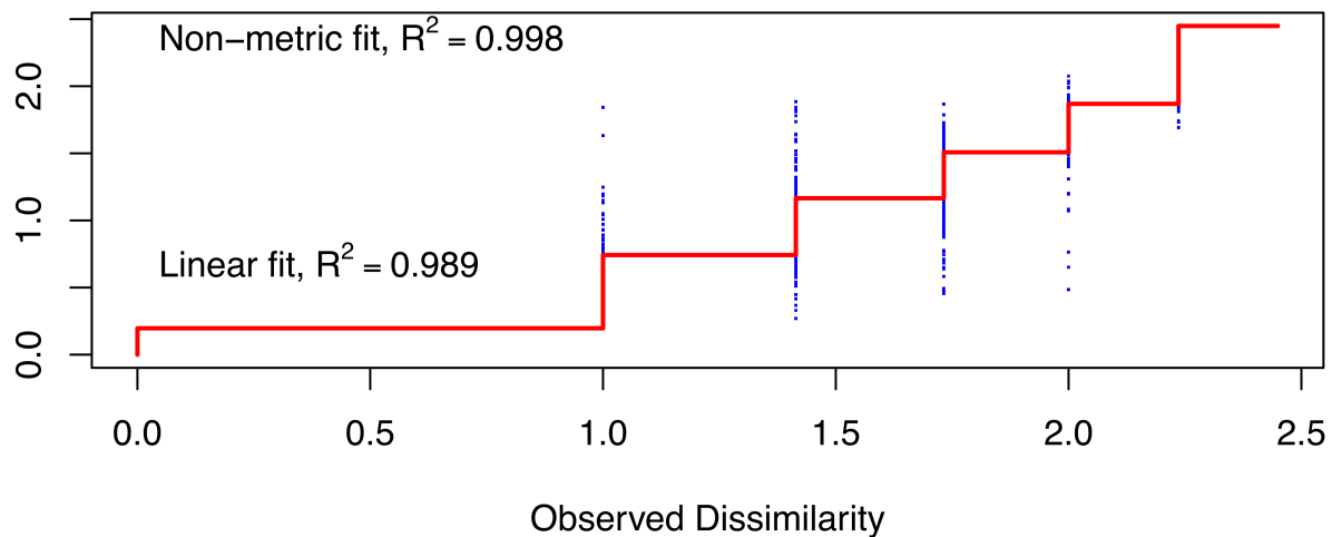
Shepards diagram
