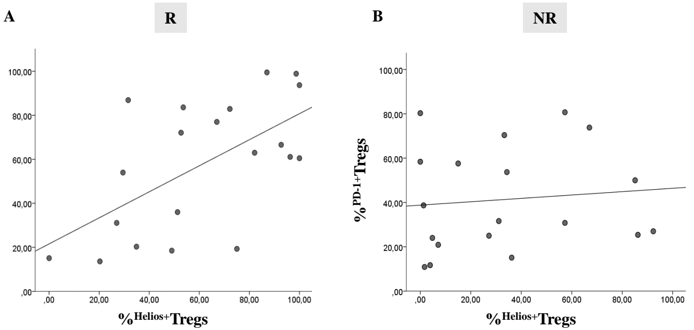
Supplementary Figure S12. Correlation between pretreatment of PD-1+Tregs and Helios+Tregs in Responder and Not-Responder patients. (A) Scatter plot of Kendall's rank correlation between pretreatment values of % Helios+Tregs and % PD-1+Tregs in Responder (Coefficient 0.396; p=0.015; N=20) and (B) Not Responder patients (Coefficient 0.125; p=0.480; N=19).
