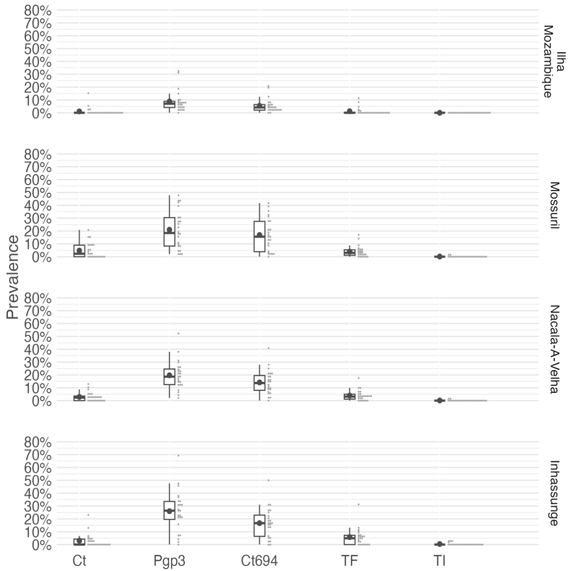
Figure S1. Distribution of cluster trachoma prevalence by district and indicator represented by box-and-whisker plots with mean cluster prevalence (dark circles) and cluster prevalence values (gray circles).
