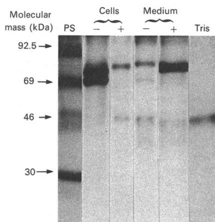
Fig. 1. SDS/PAGE and fluorography of \alpha -L-iduronidase immunopurified from normal fibroblasts
