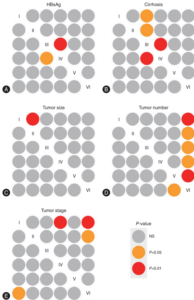
Supplementary Figure 5. Pairwise chi square analysis displays the P -value with Bonferroni adjustment in the left lower triangle and no adjustment in right upper triangle depicting the clinicopathological difference of HBsAg (A), cirrhosis (B), tumor size (C), tumor number (D) and tumor stage (E) between different stromal-immune signature.
