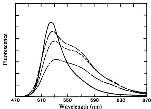
Fig. 3. Corrected fluorescence emission spectra for Rhodamine (—, 1.36 \mu\text{M} ), (Cbz-Arg-NH) 2 -Rhodamine (---, 0.10 mM), synthetic Cbz-Arg-NH-Rhodamine (— — —, 4.78 \mu\text{M} ), and trypsin-produced Cbz-Arg-NH-Rhodamine (- · - · -, 2.95 \mu\text{M} ) in 10 mM-Hepes buffer, pH 7.5, containing 15% (v/v) ethanol. The spectra are not drawn to scale.
