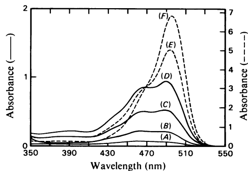
Fig. 2. Absorption spectra of the hydrolysis of (\text{Cbz-Arg-NH})_2 -Rhodamine by trypsin as a function of time. To 2 ml of 0.10 mM- (\text{Cbz-Arg-NH})_2 -Rhodamine in 10 mM-Hepes buffer, pH 7.5, containing 15% (v/v) ethanol, was added 20 \mu\text{l} of 1.2 \mu\text{M} -trypsin at time 0 and at time 126 min. Absorption spectra were recorded at the following times: A, 0 min, B, 1 min, C, 4 min, D, 9 min, E, 124 min, and F, 154 min. For spectra E and F, the absorbances were calculated from measurements on diluted solutions.
