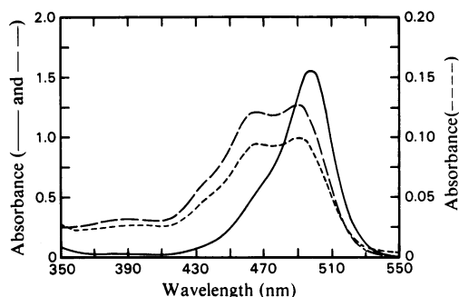
Fig. 1. Absorption spectra of Rhodamine (—, 20.6 \mu\text{M} ), synthetic Cbz-Arg-NH-Rhodamine (---, 38.1 \mu\text{M} ) and trypsin-produced Cbz-Arg-NH-Rhodamine (— · —, 2.95 \mu\text{M} ) in 10 mM-Hepes buffer, pH 7.5, containing 15% (v/v) ethanol
