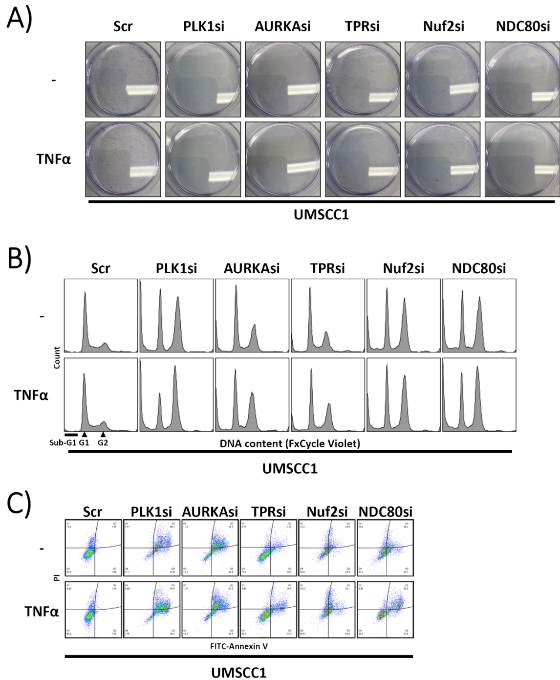
Supplementary Figure 4. Representative images from Figure 3. A) Representative images of colony formation assays in Figure 3C. B) Representative images of cell cycle analysis in Figure 3D. C) Representative images of Annexin V assay in Figure 3E.
