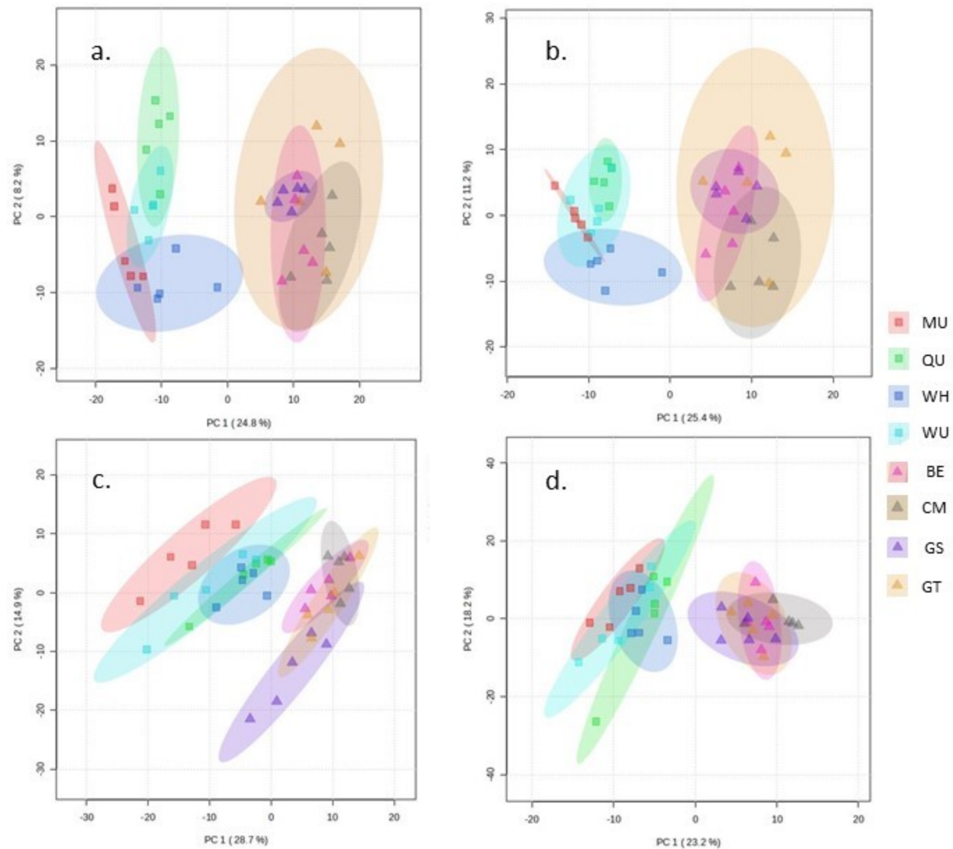
Supplementary Fig 2. Multiple PCA graphics for all NZ and SC sites in a. C18pos, b. C18neg, c. HILCpos and d. HILCneg. All demonstrate clearly separate clustering of the NZ and SC ranges. PC 1 and PC 2 demonstrate the observed variance between clusters. All analyses are validated using [PERMANOVA] p = 0.001 . Square points represent New Zealand sites and triangles represent Scotland sites.
