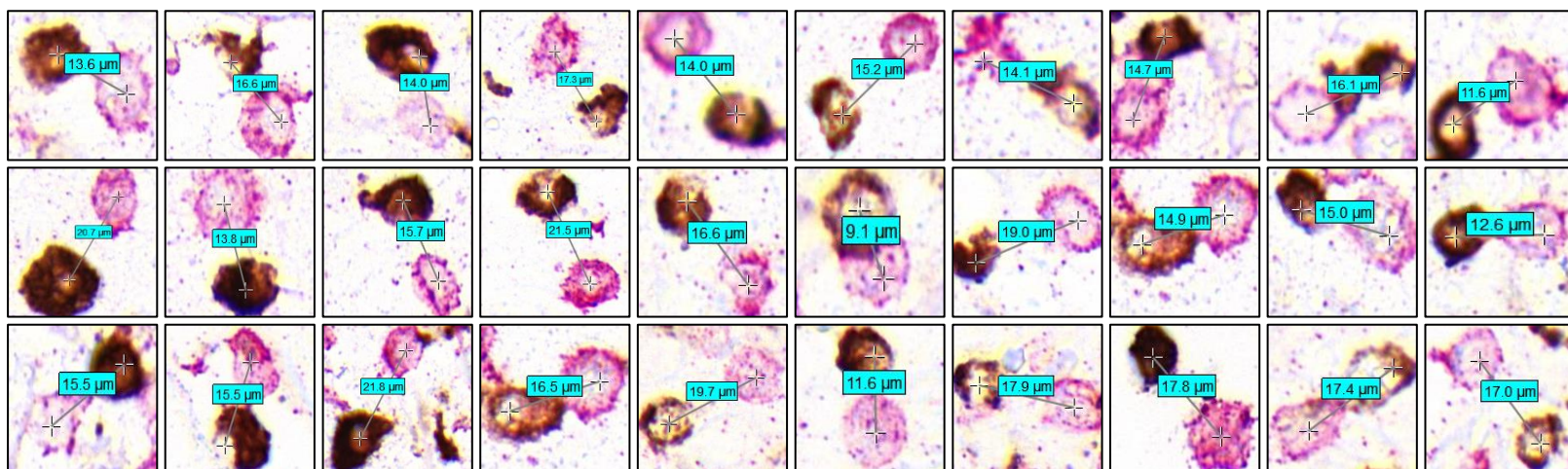
Figure S1. NK-macrophage cell distance. (A, B) The distance between decidual natural killer (NK) cells and macrophages in the decidua of normal pregnant women (A) or patients with recurrent spontaneous abortion (RSA) (B).
