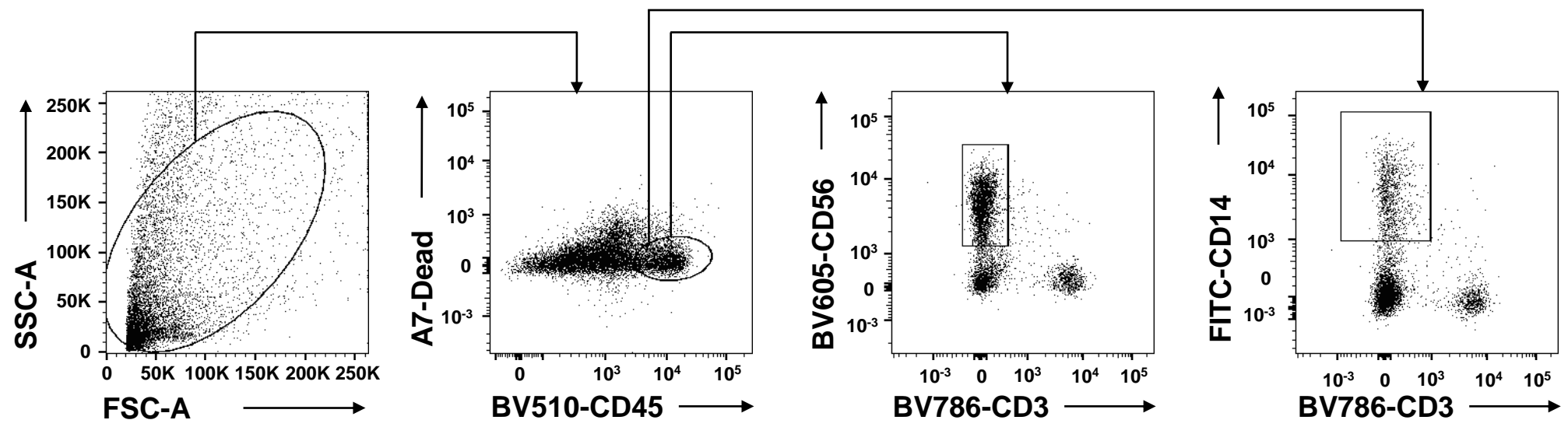
Figure S2. The gating strategy for cell sorting.
