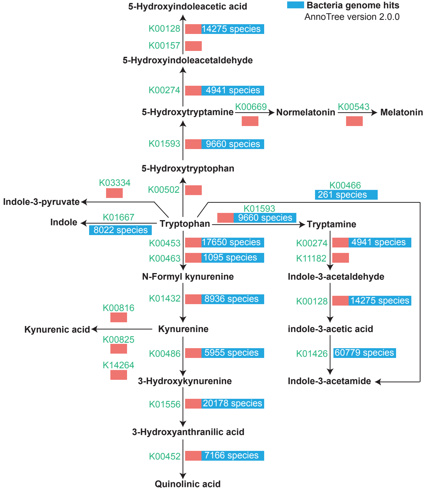
Overview of human and bacterial tryptophan metabolism pathway using the Kyoto Encyclopedia of Genes and Genomes (KEGG) pathway and AnnoTree
