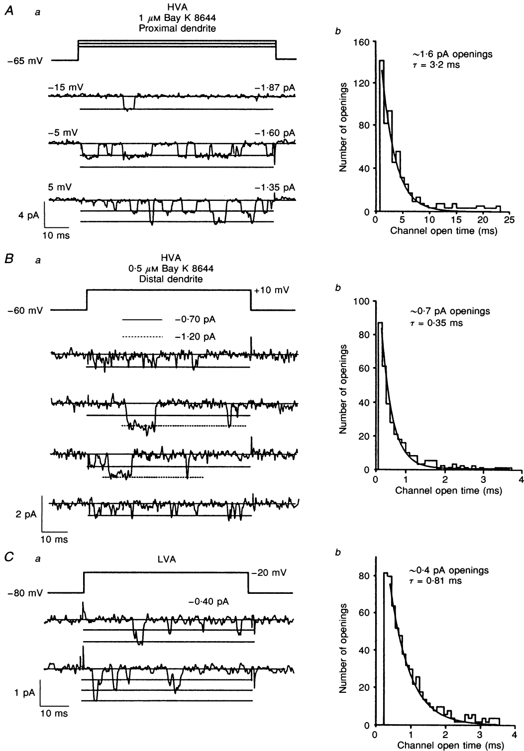
Figure 7. Effect of Bay K 8644 on dendritic \text{Ca}^{2+} channels
