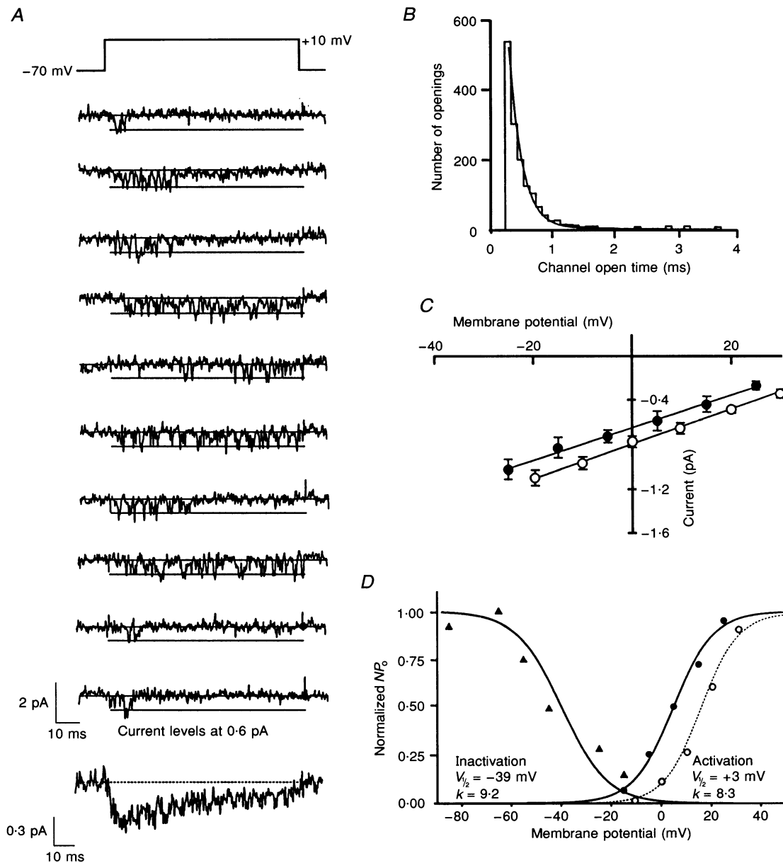
Figure 5. Dendritic high voltage-activated \text{Ca}^{2+} channel activity
